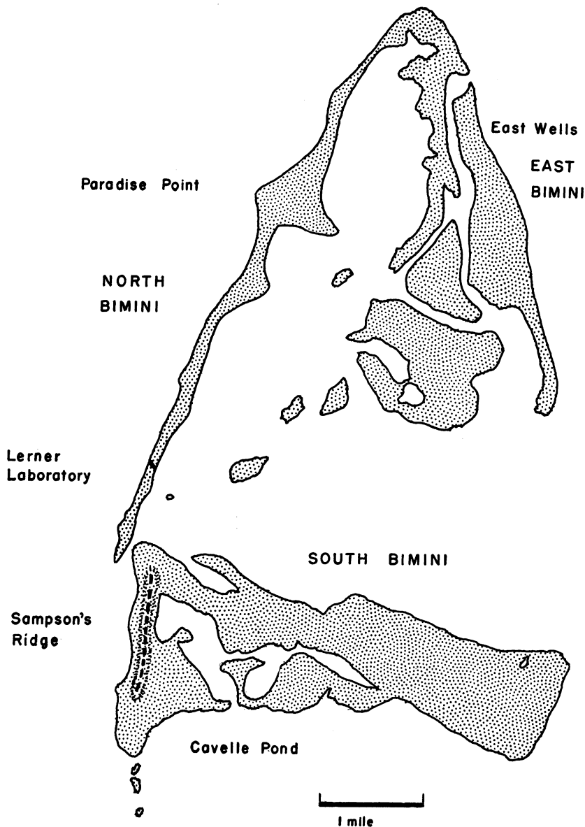
FIG. 1. Bimini island group, Bahamas.
