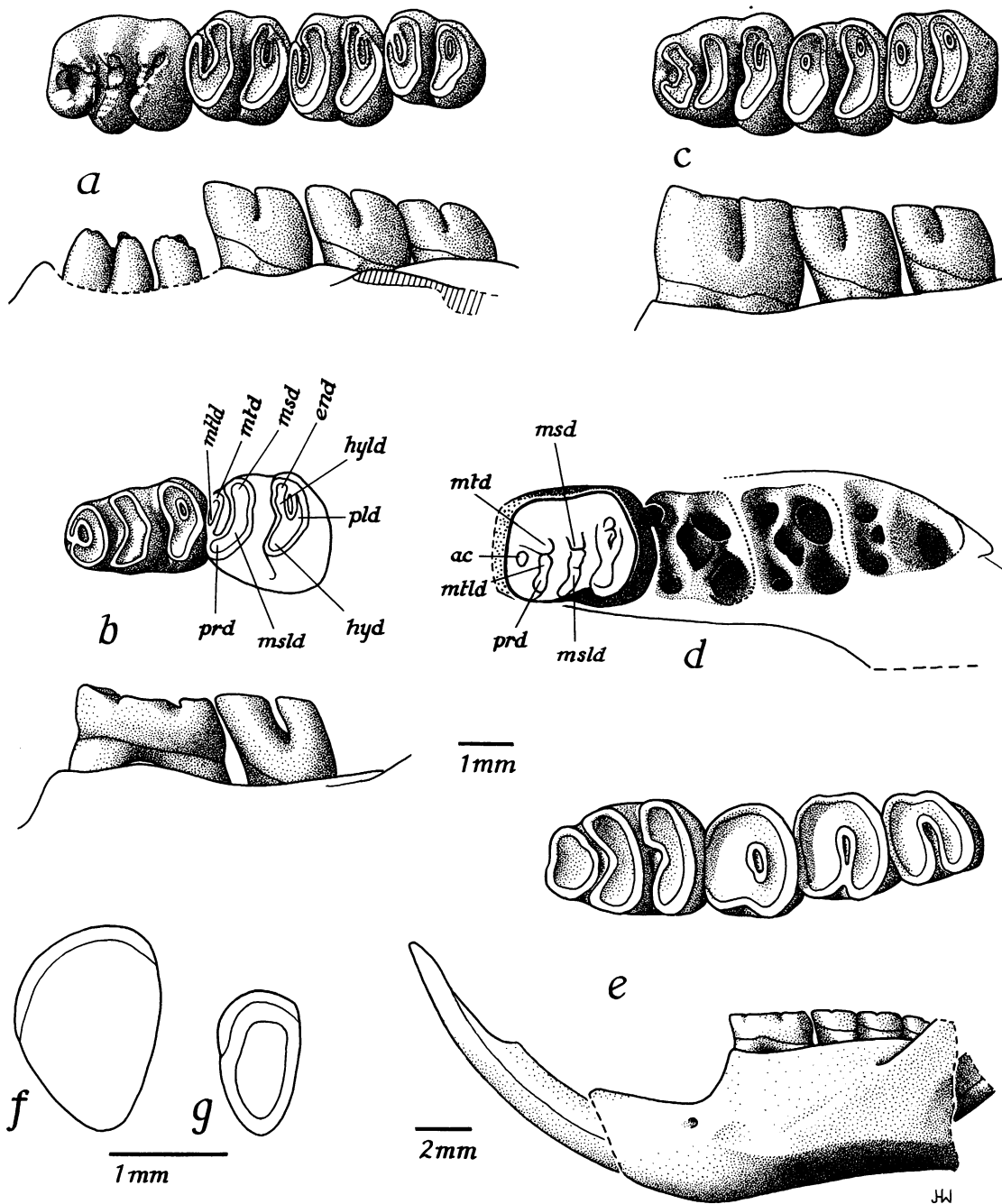
FIG. 1 a-f. Jimomys labaughi . a. F:AM 97816 (type), crown and labial views. b. F:AM 97817, crown and labial views. c. F:AM 97822, crown and labial views. d. F:AM 97820, crown view (reversed). e. 97818, crown view of teeth and labial view of jaw. f. F:AM 97816, cross section of incisor. g. Jimomys lulli , YPM 10573, cross section of incisor (reversed).
