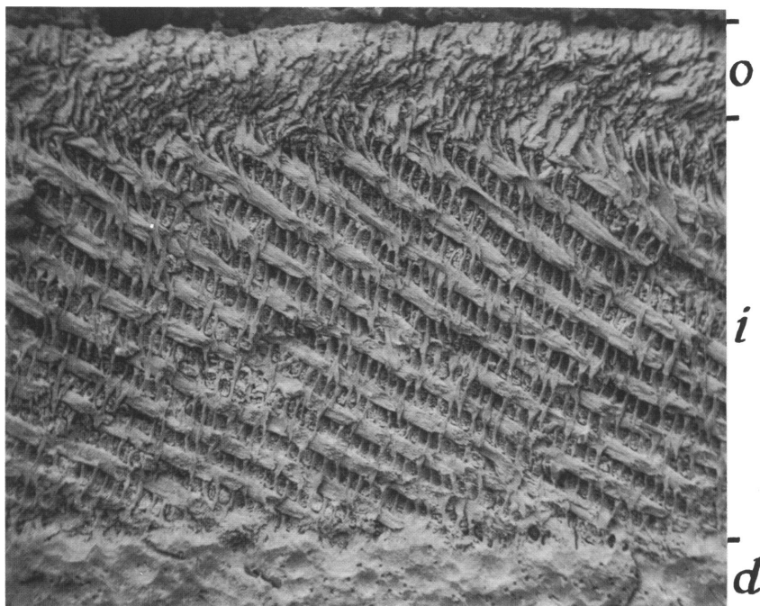
FIG. 2. Jimomys labaughi , sagittal section of incisor enamel. \times 575 . Tip of incisor is to the left.
