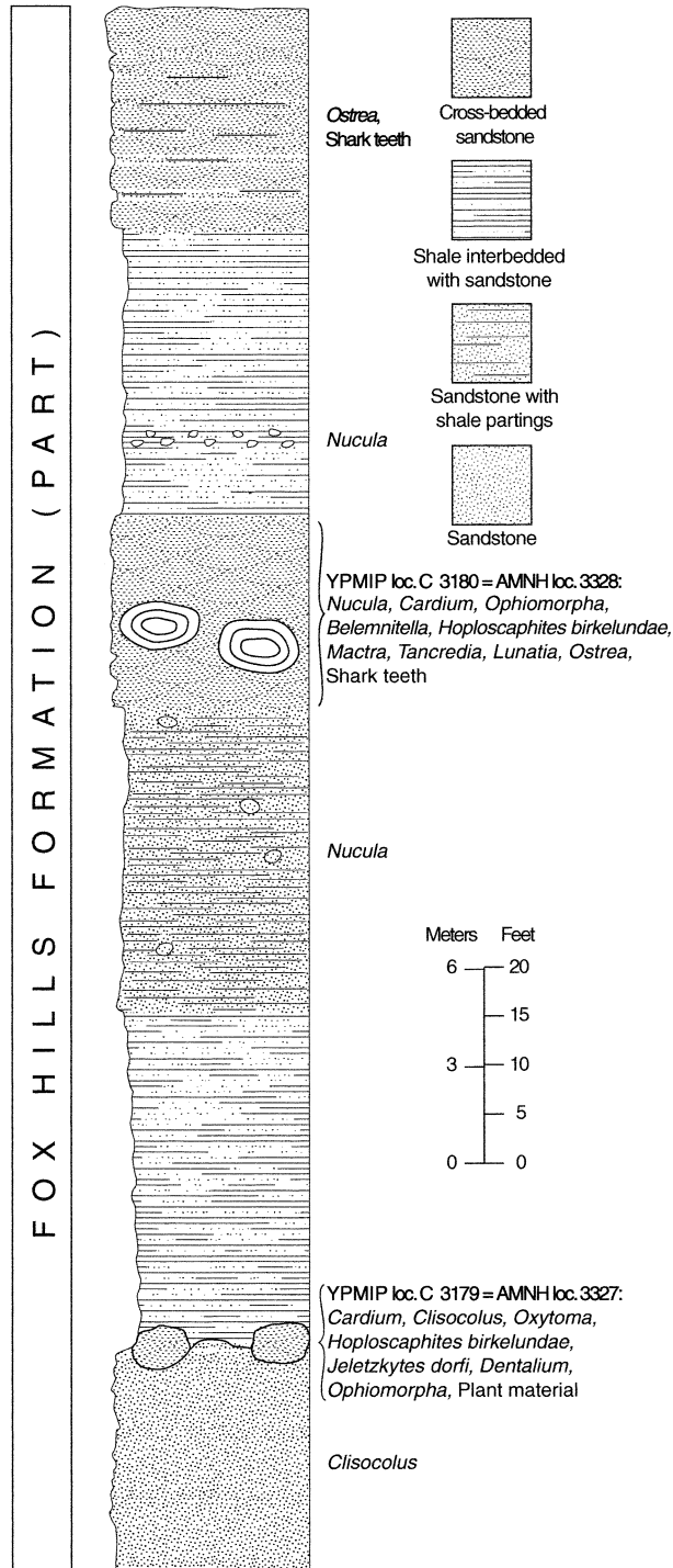
Fig. 4. Stratigraphic section of part of the Fox Hills Formation on the south side of Big Draw and the west side of Wildcat Creek, SW¼, NE¼ sec. 31, T6N, R58W, Morgan County, Colorado, as measured by K.M. Waage in 1967.
