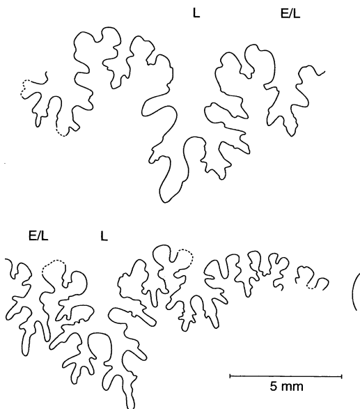
Fig. 18. Parts of two sutures of Hoploscaphites birkelundae Landman and Waage, 1993, CSM 3517, Fox Hills Formation, 13 mi (20.9 km) north of Wellington, Larimer County, Colorado. The sutures are drawn at whorl heights of 26.0 mm (above) and 18.7 mm (below).
