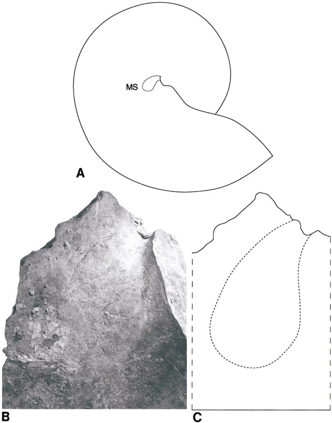
Fig. 14. Sphenodiscus pleurisepta (Conrad, 1857). A–C. USNM 519510, top of Pierre Shale or lower Fox Hills Formation, SW \frac{1}{4} , SE \frac{1}{4} sec. 35, T6N, R67W, Weld County, Colorado. A , Sketch of reconstructed specimen showing the location of the muscle scar; B , close-up of the muscle scar, \times 1.5 ; C , sketch of the muscle scar shown in B, \times 1.5 .
