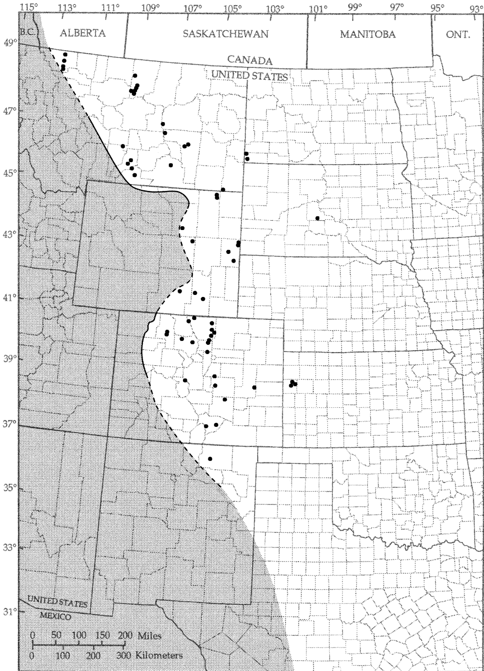
Fig. 5. Western shoreline of the Western Interior Seaway during the time of the Baculites reesei Zone (upper part of the upper Campanian). Dots indicate localities at which B. reesei occurs.
