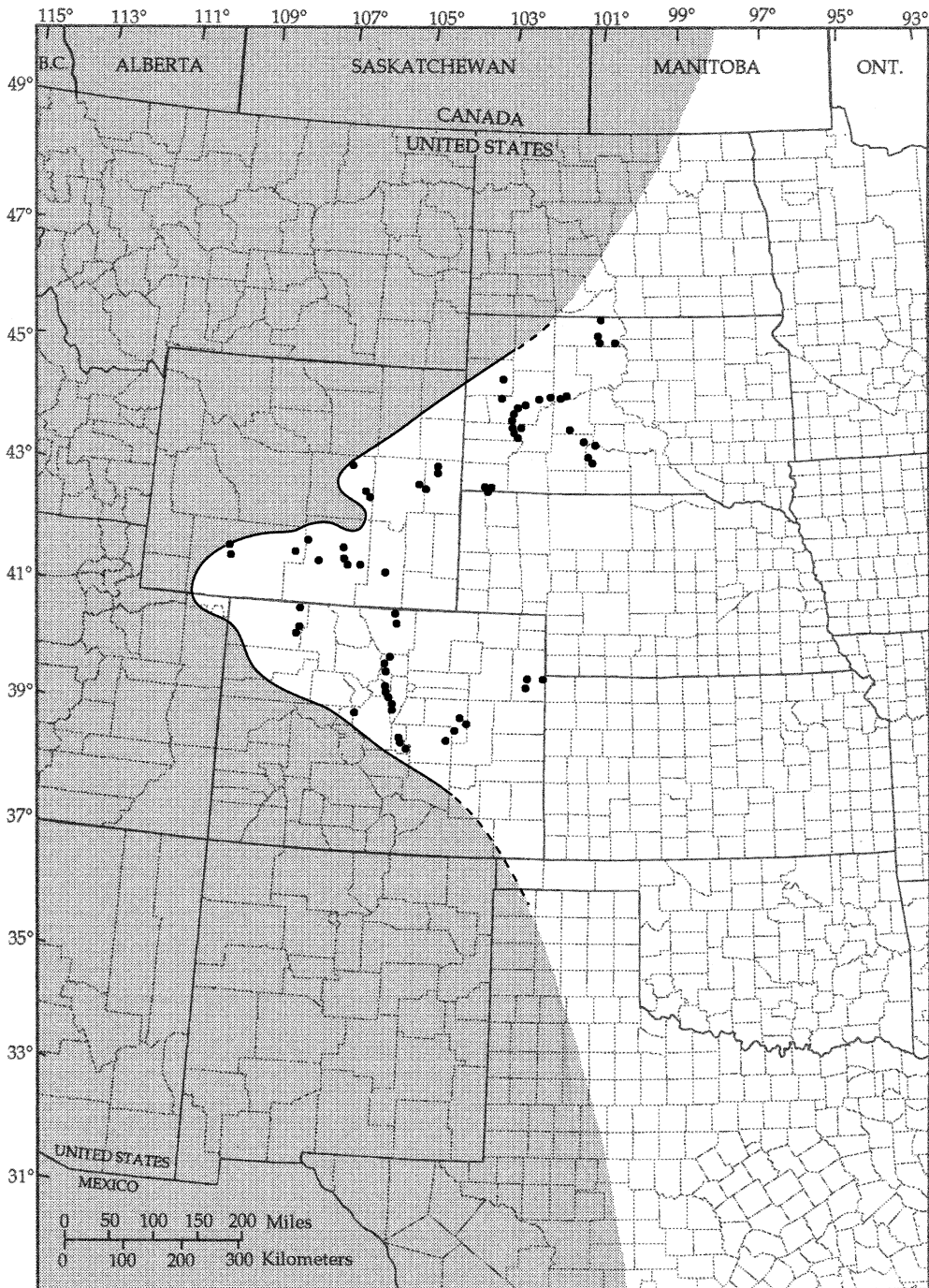
Fig. 6. Western shoreline of the Western Interior Seaway during the time of the Baculites clinolobatus Zone (upper part of the lower Maastrichtian). Dots indicate localities at which B. clinolobatus occurs. (Modified after Cobban et al., 1994: fig. 13.)
