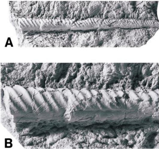
Fig. 16. Trachybaaculites sp. cf. T. columna (Morton, 1834). A , B . CSM 5612, Fox Hills Formation, near Wellington, Larimer County, Colorado. A , Right lateral, \times 1 ; B , close-up of adoral end, \times 2.8 .
