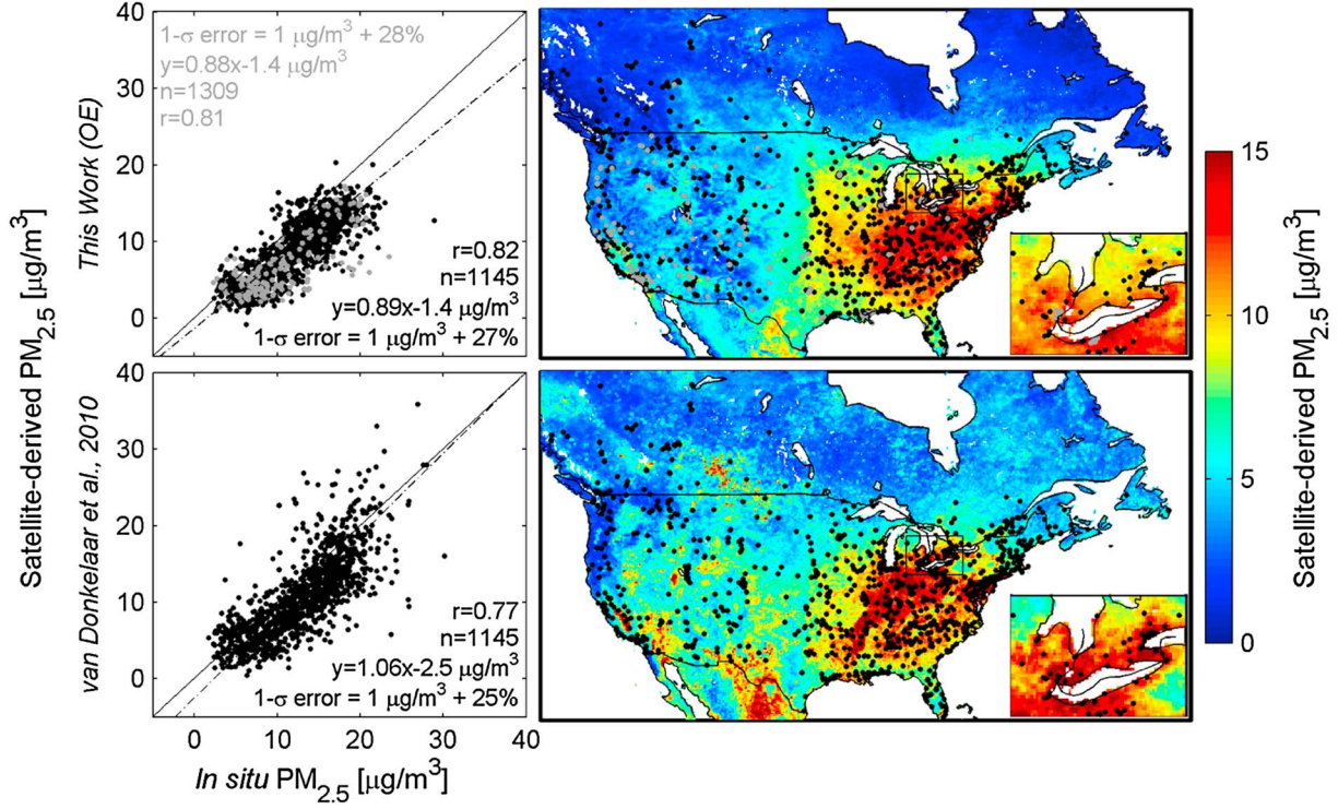
Figure 9. Comparison of satellite-derived OE PM 2.5 from this work with the previous estimates from van Donkelaar et al. [2010] for 2005. The left panels show coincidentally sampled averages at locations with at least 10 coincident in situ satellite-derived PM 2.5 pairs. The right panels show average satellite-derived PM 2.5 . Boxed regions are enlarged within the subpanel plots. Black dots indicate stations included in both scatterplots, and black text provides statistics based upon these locations alone. Grey dots indicate those additional stations that also meet minimum comparison criteria for the OE estimates. Grey text provides statistics based upon all stations available to the OE estimates. PM 2.5 estimates are at 35% relative humidity.
