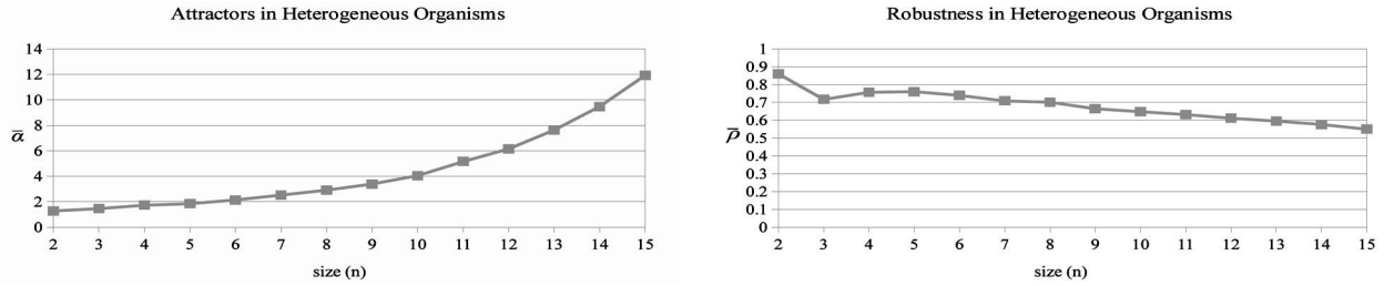
Figure 4. Attractors and robustness in heterogeneous organisms.
