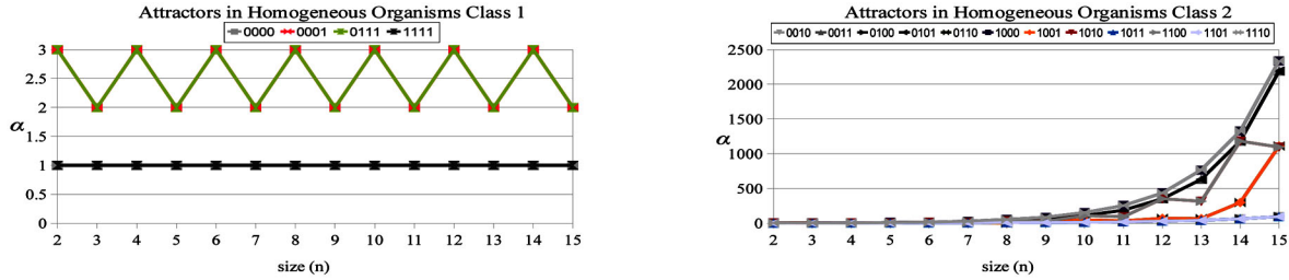
Figure 2. Homogeneous organisms with bounded (left) and unbounded (right) numbers of attractors.
