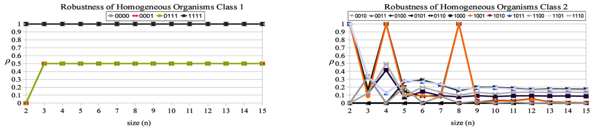
Figure 3. Robustness of homogeneous organisms of class 1 (left) and 2 (right).
