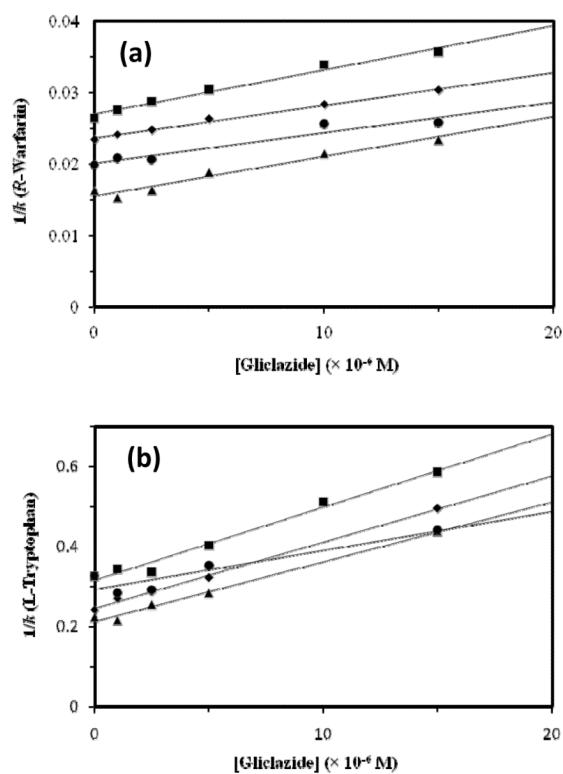
Figure 6. Plots prepared according to Eq. (6) that showing how the reciprocal of the retention factor for (a) R -warfarin or (b) L -tryptophan changed on HSA or glycosylated HSA columns as the concentration of gliclazide was varied in the mobile phase. These results are for normal HSA (◆), gHSA1 (■), gHSA2 (▲), and gHSA3 (●).
