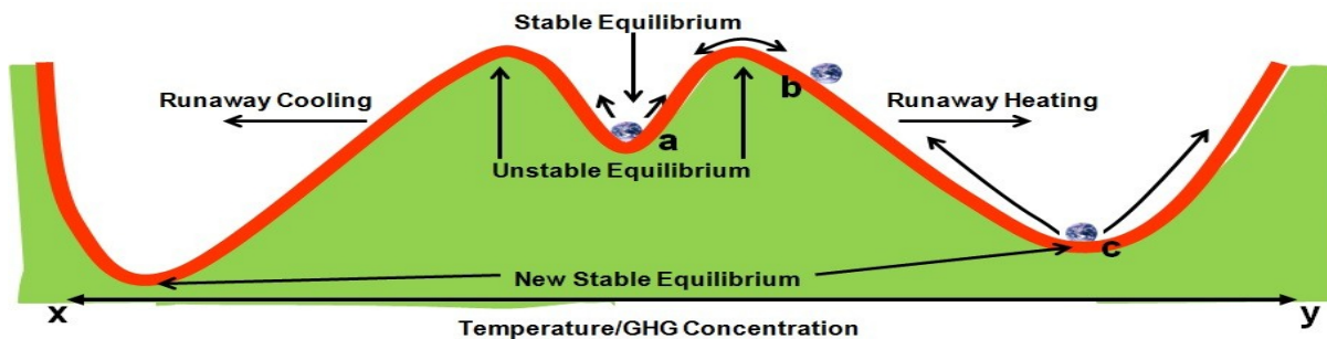
Figure 4: Topographic cross-section of possible climate states (derived from Wasdell, "Feedback" 26 CC).
