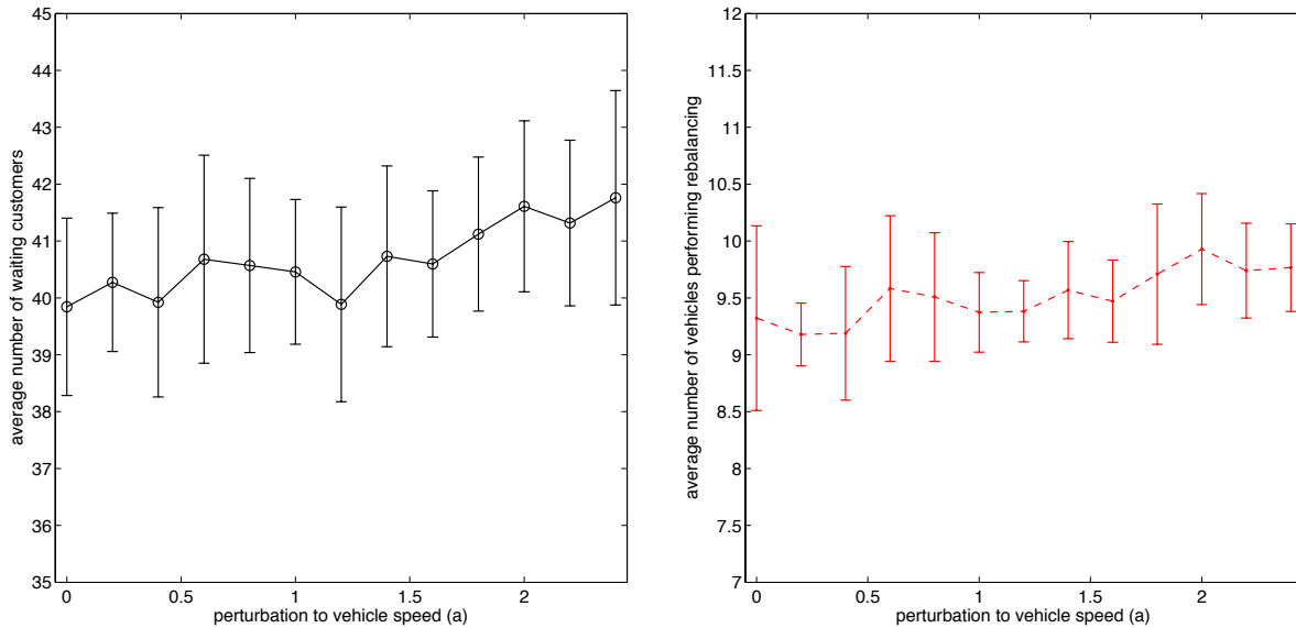
Figure 7: The performance of the real-time rebalancing policy as a function of uncertainty on travel-times. The nominal vehicle step size is 0.2, and a zero mean uniform random variable U(-a, a) is added to the step size at each time step. The value of a is shown on the x -axis of the plot, ranging from 0 to 2.4. Left figure: The time-average number of customers waiting in the system. Right figure: The time-average number of vehicles performing rebalancing trips.
