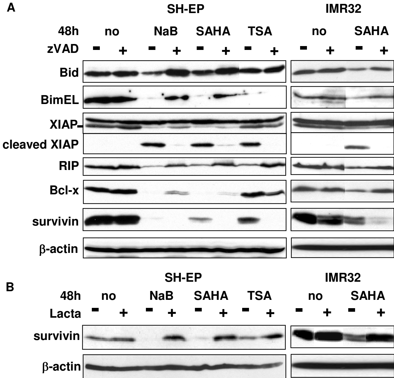
Figure 5 HDACi increase the pro- to anti-apoptotic protein ratio by different mechanisms. A. SH-EP cells were unstimulated (no), or stimulated with NaB (20 mM), SAHA (20 \mu M) or TSA (5 \mu M) in the absence (-) or in the presence (+) of zVAD-fmk for 48 h. IMR32 cells were unstimulated (no) or stimulated with 2.5 \mu M of SAHA in the absence (-) or in the presence (+) of zVAD-fmk for 48 h. Whole cell extracts were analysed by immunoblotting with anti-Bid, Bim, XIAP, RIP, Bcl-x L survivin antibodies. B. SH-EP cells were unstimulated (no), or stimulated with NaB, SAHA or TSA in the absence (-) or in the presence (+) of Lactacystin (10 \mu M) as in (A). IMR32 were unstimulated (no) or stimulated with SAHA (5 \mu M) in the absence (-) or in the presence (+) of Lactacystin (10 \mu M) for 48 h. Whole cell extracts were analysed for the presence of survivin. \beta -actin was used as loading control (A and B).
