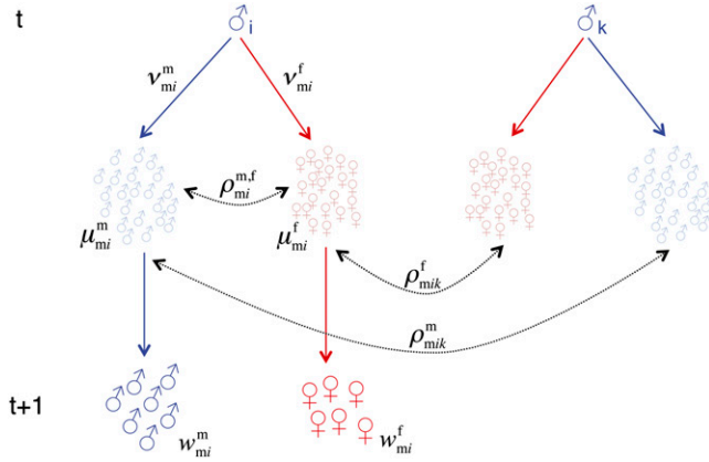
Figure 1 The moments of male reproduction. At generation t , a focal male i sires an expected \mu_{mi}^m number of male offspring with variance \nu_{mi}^m and covariance \rho_{mik}^m with the number of male offspring sired by another male k . The males of the next generation t + 1 are established by sampling the juveniles and the expected number of adult males of the focal male i is w_{mi}^m . Similarly, the focal male sires an expected \mu_{mi}^f number of female offspring with variance \nu_{mi}^f and covariance \rho_{mik}^f with the number of females sired by male k . Then, the expected number of adult females of the focal male i is w_{mi}^f . Finally, the number of male and female offspring of male i covary by \rho_{mi}^{m,f} .
