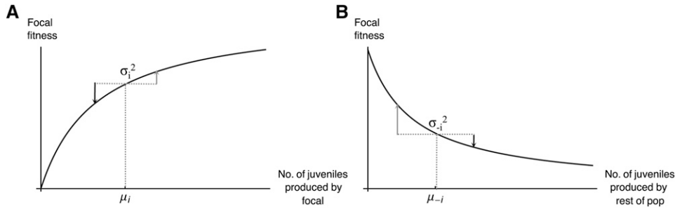
Figure 2 Effects of variance on focal fitness. (A) Fitness of a focal individual graphed against the random number of offspring it produces and holding the rest of the population constant. Ignoring the sex of parent and offspring, the focal produces on average \mu_i offspring with variance \sigma_i^2 . It then produces more or less than \mu_i offspring. But fitness is a relative measure of reproductive success (Equation 3). The advantage of producing more offspring depreciates with the
