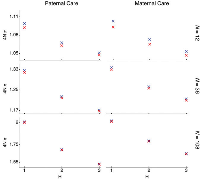
Figure 5 Approximate probabilities of fixation of parental care strategies against harem size. The probabilities of fixation scaled to the total gene number, 4N\pi , of paternal (first column) and maternal (second column) care are shown for populations with N = 12 (first row), N = 36 (second row), and N = 108 (third row) males and females against harem size H . Care for sons is shown in blue and care for daughters in red. The monogamous case corresponds to H = 1 . Other parameters are set at f = 10 , s = 0.3 , and \delta = 0.01 .
