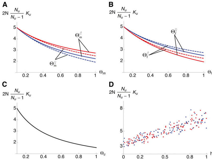
Figure 4 The effect of probabilities of sibship and dominance on the weights K_m and K_f . The effects of the probabilities that two males (A) and two females (B) and that a male and female (C) are sibs are shown for an additive mutant (Equation A2) when all the other probabilities of sibship are fixed at 0.1. In A and B, K_m is shown in blue and K_f is shown in red. How they change with the paternal ( \Theta^\sigma ) and maternal ( \Theta^\omega ) probabilities of sibship is shown as solid and dashed lines respectively. In C, the effects of paternal ( \Theta^\sigma ) and maternal ( \Theta^\omega ) probabilities of sibship on K_m and K_f are equal and shown as a single solid line. In D, we solved for K_m (blue) and K_f (red) (File S1, Equation S1.38) for 100 different values of dominance h , with probabilities of sibship randomly perturbed around 0.1 (each probabilities of sibship was sampled from a normal distribution with mean 0.1 and variance 0.02).
