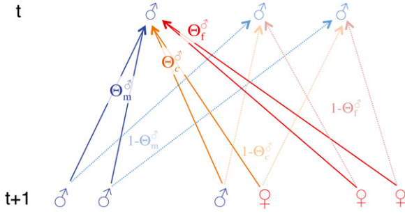
Figure 3 The paternal probabilities of sibship. With probability \Theta_m^\sigma , two males sampled at generation t + 1 have the same father from generation t . So, with probability 1 - \Theta_m^\sigma , they come from different fathers. Similarly, a male and a female sampled at generation t + 1 have the same father with probability \Theta_c^\sigma , and two females do so with probability \Theta_f^\sigma .
