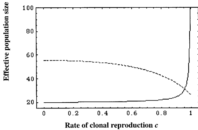
FIGURE 5.—Allelic effective population size (solid line) and genotypic effective population size (dashed line) in a non-subdivided population. The values given are for a population of 20 individuals.
