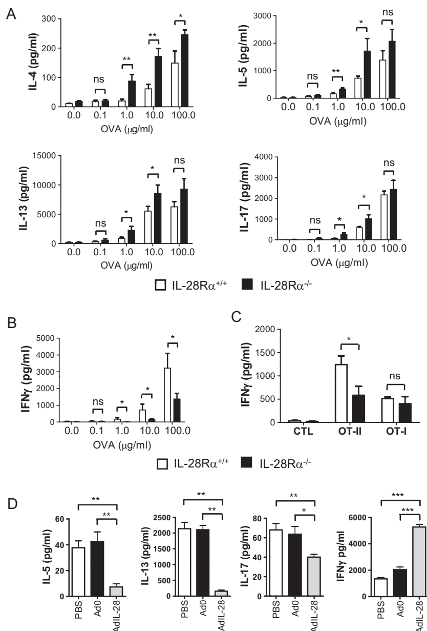
Figure 4. IL-28 signalling is required for skewing T helper cell differentiation to a Th1 cytokine profile.
