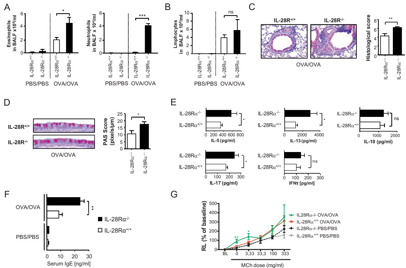
Figure 3. IL-28R \alpha -deficient mice develop increased Th2/Th17 responses and Th2/Th17-mediated allergic airway inflammation.
