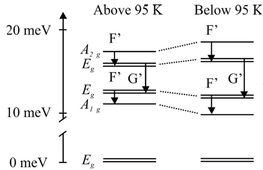
FIG. 5. Schematic of the crystal field levels in \text{Ho}_2\text{Ru}_2\text{O}_7 (adapted from Rosenkranz et al. [20]). The transitions F' and G' are noted. As the \text{Ru}^{4+} moments order, the crystal fields are split slightly. The schematic is not to scale and the splitting is exaggerated for clarity.
