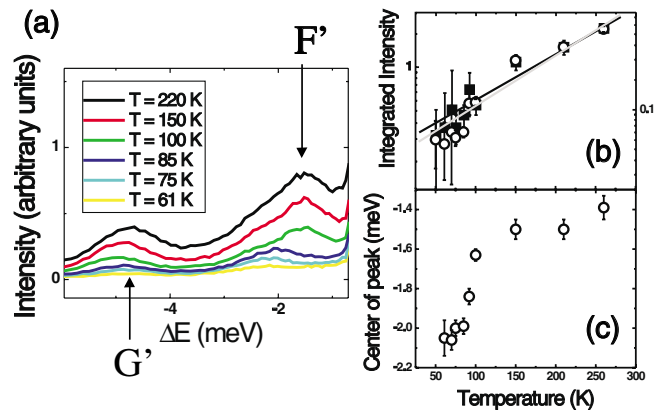
FIG. 4 (color online). (a) Integrated scans from |Q| = 0.6 to 4.0 \text{ \AA}^{-1} . Note the crystal field transitions, indicated by F' and G' . (b) Integrated intensities of the crystal field peaks, as fit to Gaussians, as a function of temperature. The open circles (gray fit) belong to the left scale ( F' transitions) and the closed squares (black fit) belong to the right ( G' transitions). (c) Shift of the center of the Gaussian peak for F' transitions.
