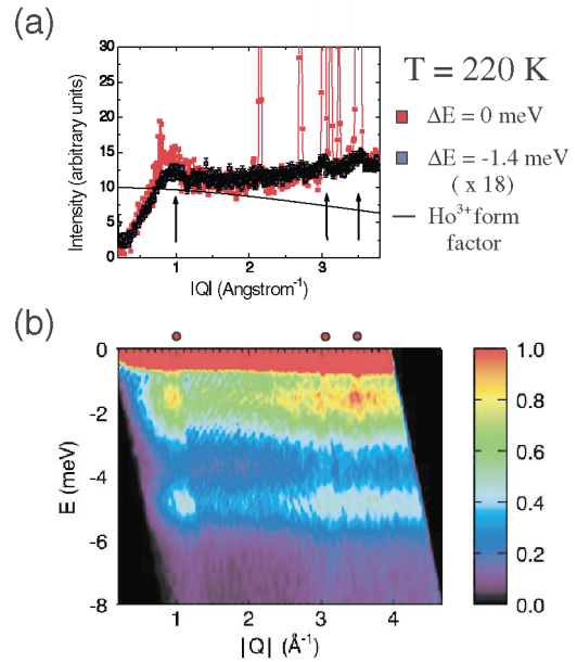
FIG. 3 (color online). (a) Integrated neutron scattering data at energy transfers of 0 and -1.4 \text{ meV} and at 220 K (with a width of 0.6 \text{ meV} ) with the DCS and neutrons of \lambda \sim 3 \text{ \AA} . The positions of the (111), (422), and (440) reflections are noted, as well as the \text{Ho}^{3+} form factor. (b) Neutron scattering contour plot at T = 220 \text{ K} , showing dispersionless features at -1.4 and -4.8 \text{ meV} [24].
