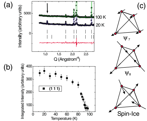
FIG. 1 (color online). (a) Neutron scattering with 2.37 \text{ \AA} neutrons at T = 100 and 20 K. The fits are to the crystal structure of \text{Ho}_2\text{Ru}_2\text{O}_7 (upper tick marks) and a magnetic structure ( \psi_7 and \psi_8 ) described in the text. The residual of the 20 K fit is at the bottom of the plot ( R_p = 1.99 , R_{wp} = 2.69 , \chi^2 = 2.02 at 100 K; R_p = 2.82 , R_{wp} = 3.73 , R_{\text{mag}} = 40.9 , \chi^2 = 3.73 at 20 K). (b) The integrated intensity of the magnetic (111) reflection [as indicated in (a)]. (c) \psi_7 and \psi_8 of the IR \Gamma_9 , and the spin-ice state which arises from equal proportions of these basis vectors.
