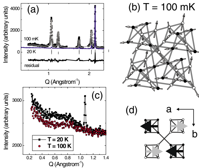
FIG. 2 (color online). (a) The diffraction data, fit (gray line) and residual (black line) for 2.0775 \text{ \AA} neutrons at 100 mK. The upper tick marks are for the crystal structure and the lower for the magnetic ( R_p = 6.06 , R_{wp} = 7.85 , R_{\text{mag}} = 8.62 , \chi^2 = 4.35 ). The 20 K neutron data (blue line) is normalized to the (222) predominantly nuclear reflection. (b) The magnetic structure of the Ru moments (black) and Ho moments (gray) at 100 mK. For clarity, only a portion of the unit cell is shown, and the ordered moments are not drawn to scale. (c) Diffraction data with 2.37 \text{ \AA} neutrons at T = 20 and 100 K, showing an intermediate state of SRO \text{Ho}^{3+} above 1.4 K. (d) The magnetic structure at 100 mK can be thought of as a nearly collinear ferromagnet (Ru sites, in black) and a spin-ice-like state (Ho sites, in gray) upon the different sublattices. The net moment cancels from one sublattice to the next along one crystallographic direction.
