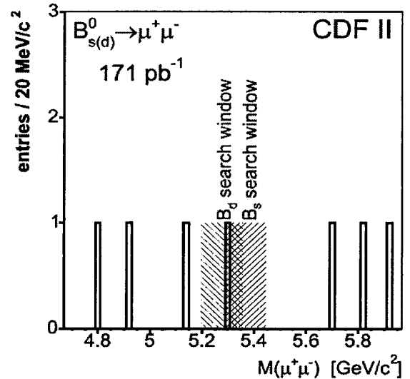
FIG. 2. The \mu^+ \mu^- invariant mass distribution of the events in the sideband and search regions satisfying all requirements.
