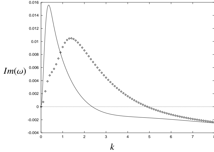
Figure 7: Growth rates plotted against k for a case where long waves are unstable and short stable, c = \infty (UCM), \kappa = 0.5 , W_1 = 5 , W_2 = 0 . Outer fluid more elastic, fastest growing mode is sinuous with k \sim 0.5 . The first peak is the sinuous mode, and the points show the varicose mode.
