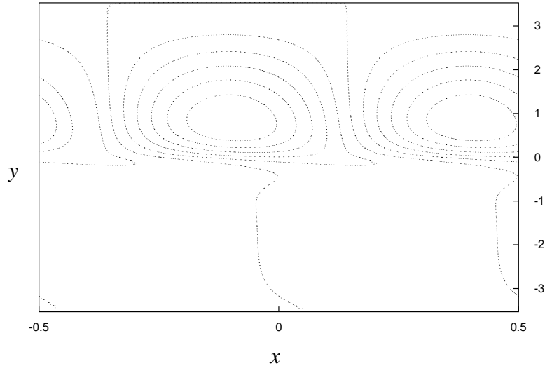
Figure 4: Streamlines of perturbation to Couette flow; stable case. c = \infty (UCM), W_2 = 5 .
