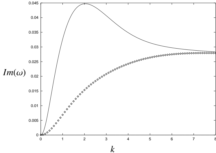
Figure 6: Growth rates plotted against k for a case where both long and short waves are unstable, c = 0.2 , \kappa = 0.5 , W_1 = 4 , W_2 = 0 . Outer fluid more elastic, fastest growing mode is sinuous with k \sim 2 . The solid curve is the sinuous mode, the points show the varicose mode.
