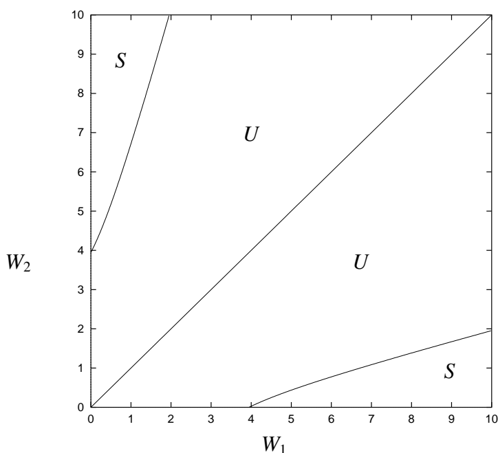
Figure 2: Neutral stability curves for c = \infty , k = \infty , \kappa = 1/2 . U , unstable; S , stable [7]. There is stability if W_1 = W_2 or if W_1 and W_2 are very different from each other. Elsewhere the interface is unstable.
