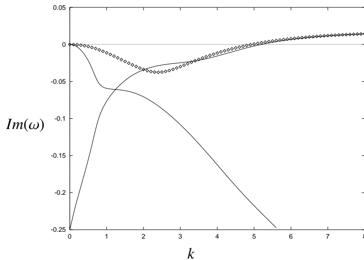
Figure 8: Growth rates plotted against k for a case where long waves are stable and short unstable, c = 0.2 , \kappa = 0.5 , W_1 = 0 , W_2 = 4 . Inner fluid more elastic, fastest growing mode has k = \infty . The varicose mode (points) almost always has the higher growth rate; two different sinuous modes are shown (solid lines).
