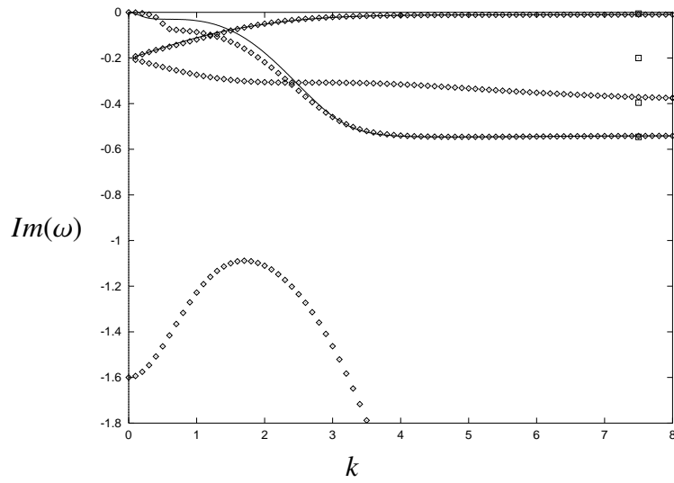
Figure 9: Growth rates plotted against k for a case where both long and short waves are stable, c = \infty (UCM), \kappa = 0.5 , W_1 = 0 , W_2 = 5 . Inner fluid more elastic; all modes decay. The sinuous modes are solid lines, the points are the varicose modes. In the short-wave limit, the dispersion relation is a polynomial which has five roots [7], four of which are marked here with small squares. The fifth has a decay rate of 5.8, and is not visible on the scale of this graph. For varicose modes we were unable to determine solutions along four of the known solution branches beyond k_c \sim 3.5 .
