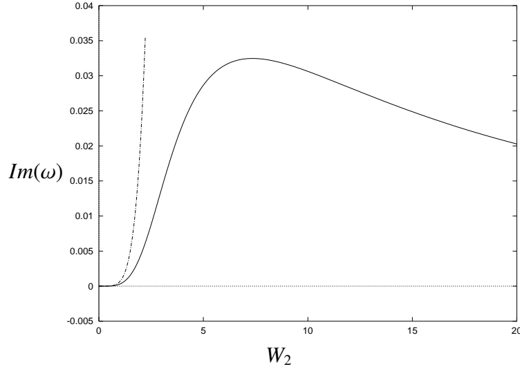
Figure 5: Growth rate against W_2 when c = 0.2 , W_1 = 0 ; the dotted curve is the asymptote found for the theory of 4.3. As W_2 \rightarrow \infty , the growth rate is proportional to 1/W_2 but the coefficient is not known analytically.
