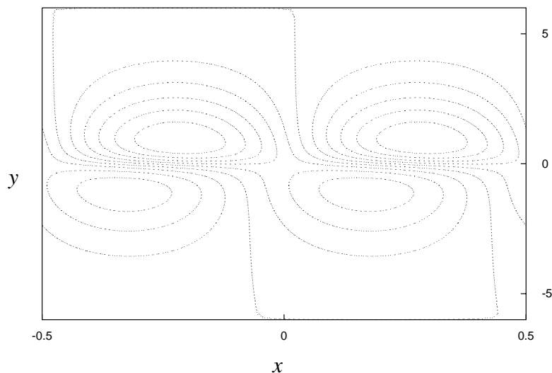
Figure 3: Streamlines of perturbation to Couette flow; unstable case. c = 0.2 , W_2 = 5 .
