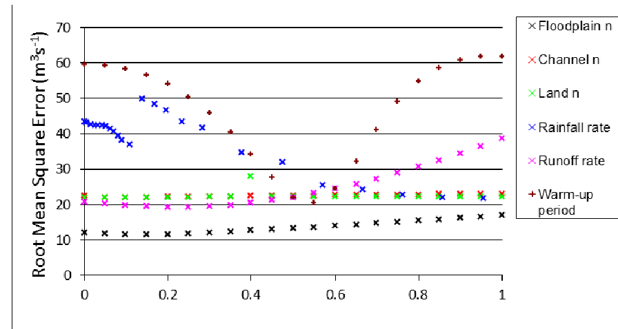
Figure 5.15b. Variation in Root Mean Square Error against a normalised parameter scale. Rain time map fixed at 180 mm/day for roughness parameters
