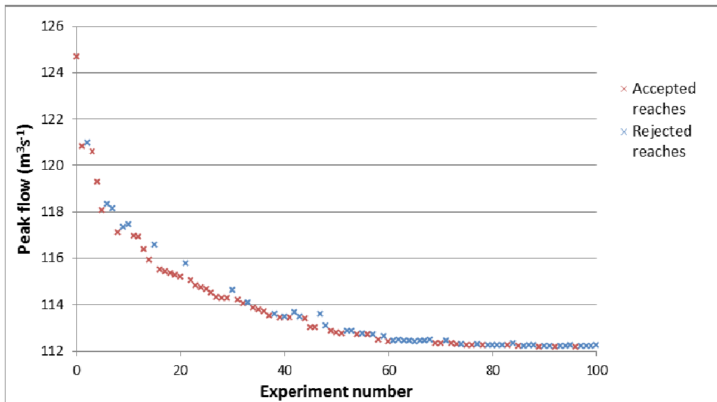
Figure 8.16. A scatter plot showing the cumulative effect on the flood peak just upstream of Uckfield of adding CRIMs to numerous reaches throughout the catchment. Experiment number also relates to the ranking of positive reaches so that the point at 1 on the x axis shows flow peak after adding a CRIM to the reach with the largest effect on the flow peak. Point 2 shows the effect of combining CRIMs at the 2 reaches with the largest effect. Points in blue indicate a decrease in cumulative downstream peak flow reduction; these reaches were rejected.
