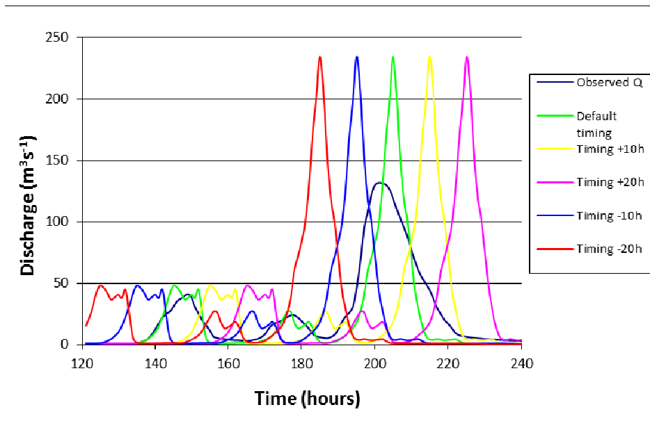
Figure 5.19b. 180 mm/day time map
