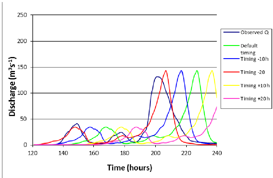
5.19a. 30 mm/day time map
