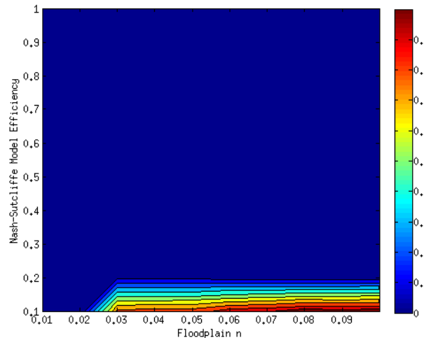
Figure 6.9a. PDF of Nash-Sutcliffe Model Efficiency against Floodplain Manning's n
