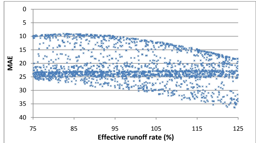
Figure 6.2b. Dotty plot of Mean Absolute Error against effective runoff %.
