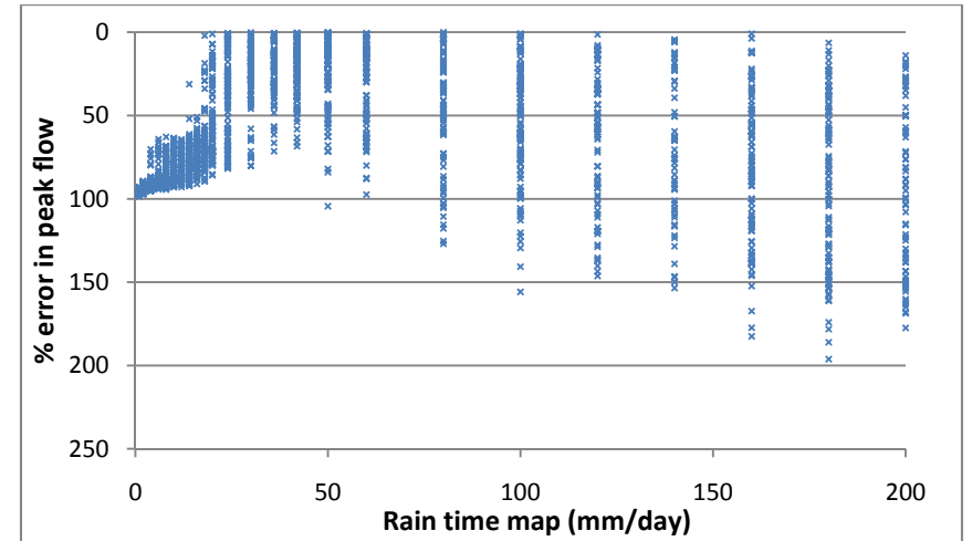
Figure 6.1d. Dotty plot of % error in peak flow against rain time map.
