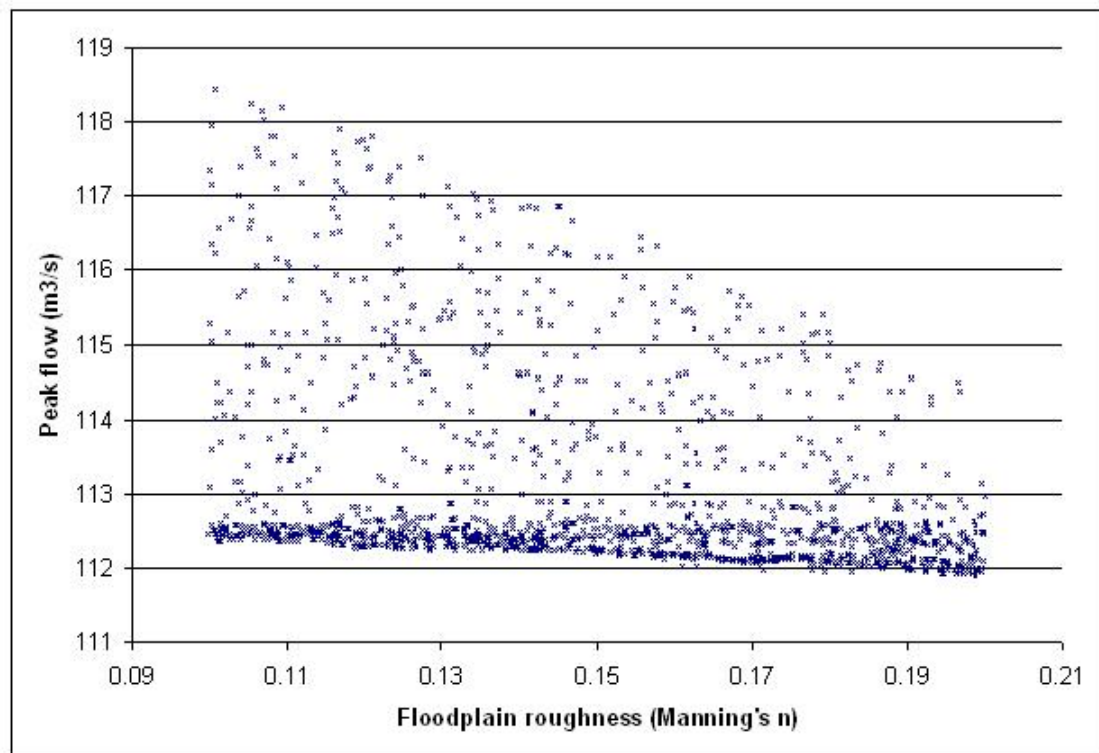
Figure 2. Each data point represents 1 model simulation where floodplain and channel roughness was randomly selected along the 52 reaches previously identified
