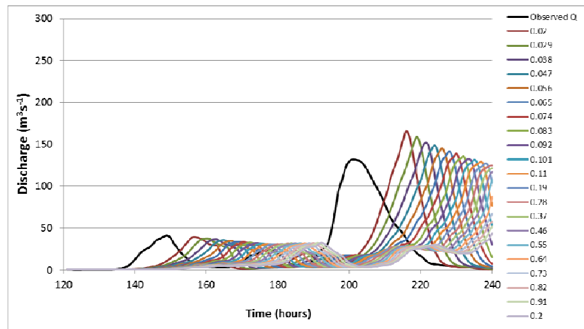
Figure 5.6. The hydrographs simulated as floodplain Manning's n is varied from 0.02 to 0.2. The hydrograph in black shows the observed discharge at Isfield during the 2000 flood event. Rain time map set at 30 mm/day.
