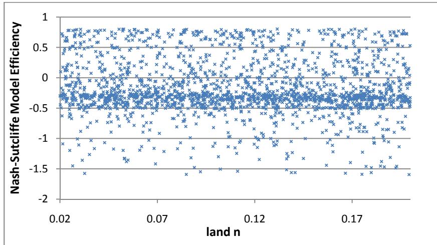
Figure 6.5a. Dotty plot of Nash-Sutcliffe Model Efficiency measure against land manning's n.
