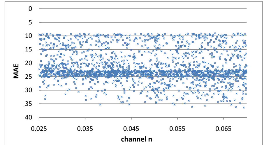
Figure 6.3b. Dotty plot of Mean Absolute Error against channel Manning's n .
