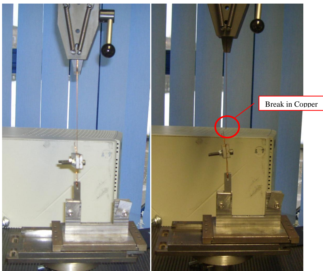
Figure 51 Photographs of Copper Wire test set-up
