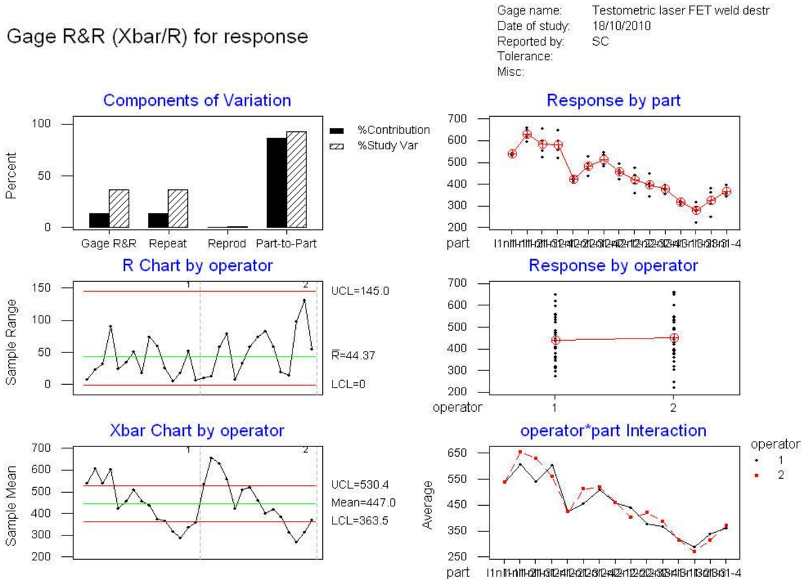
Figure 42 Destructive Gage R&R for the experimental shear test
