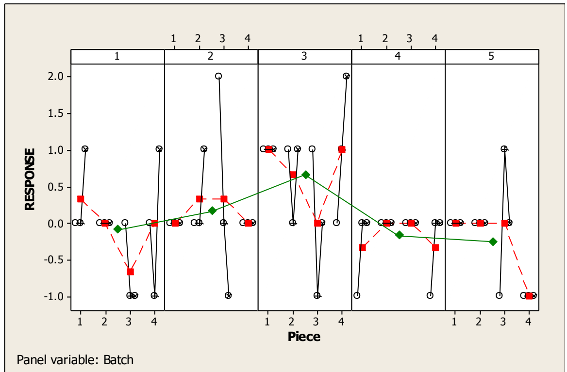
Figure 14 Shainin Multi-Vari Study for Edge 2, showing Red X^{SM} as within-piece
