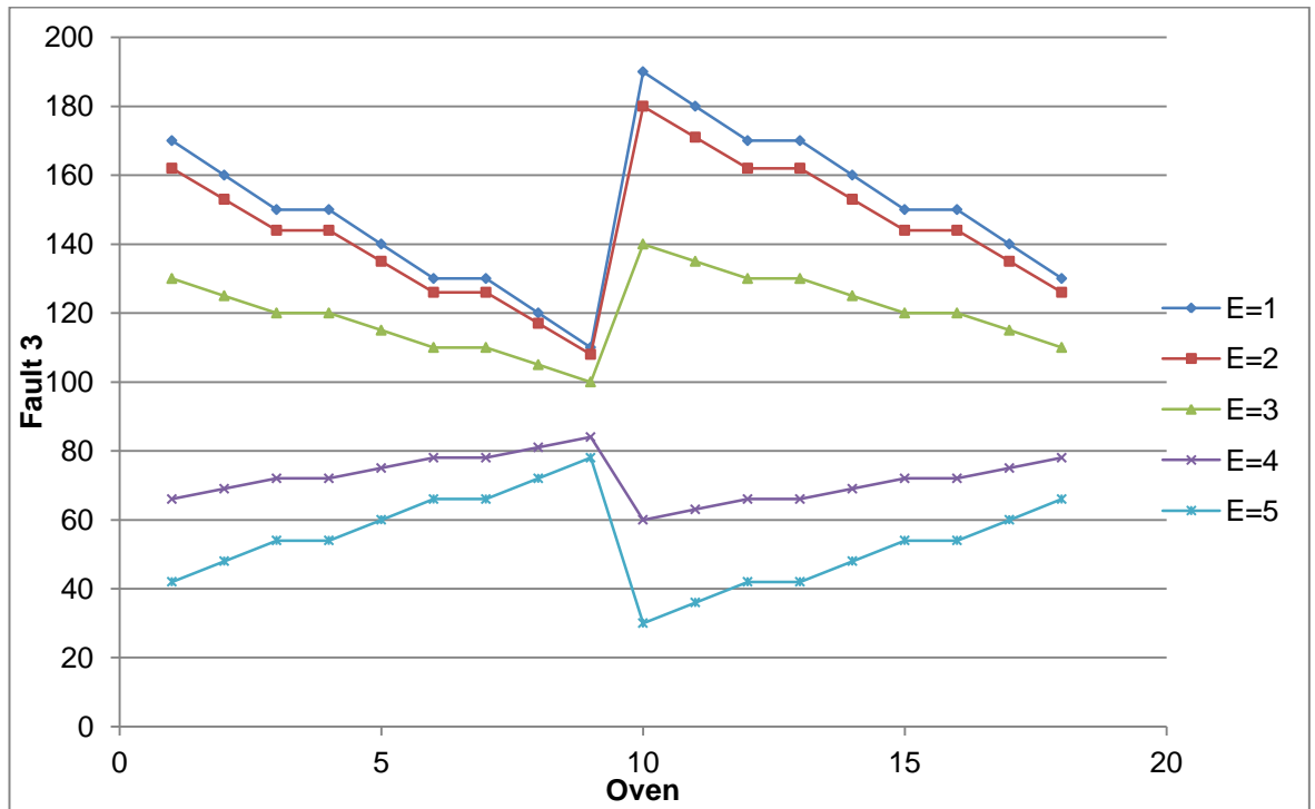
Figure 37 Distribution of Fault 3, Plotting Oven*E interaction from (10)
