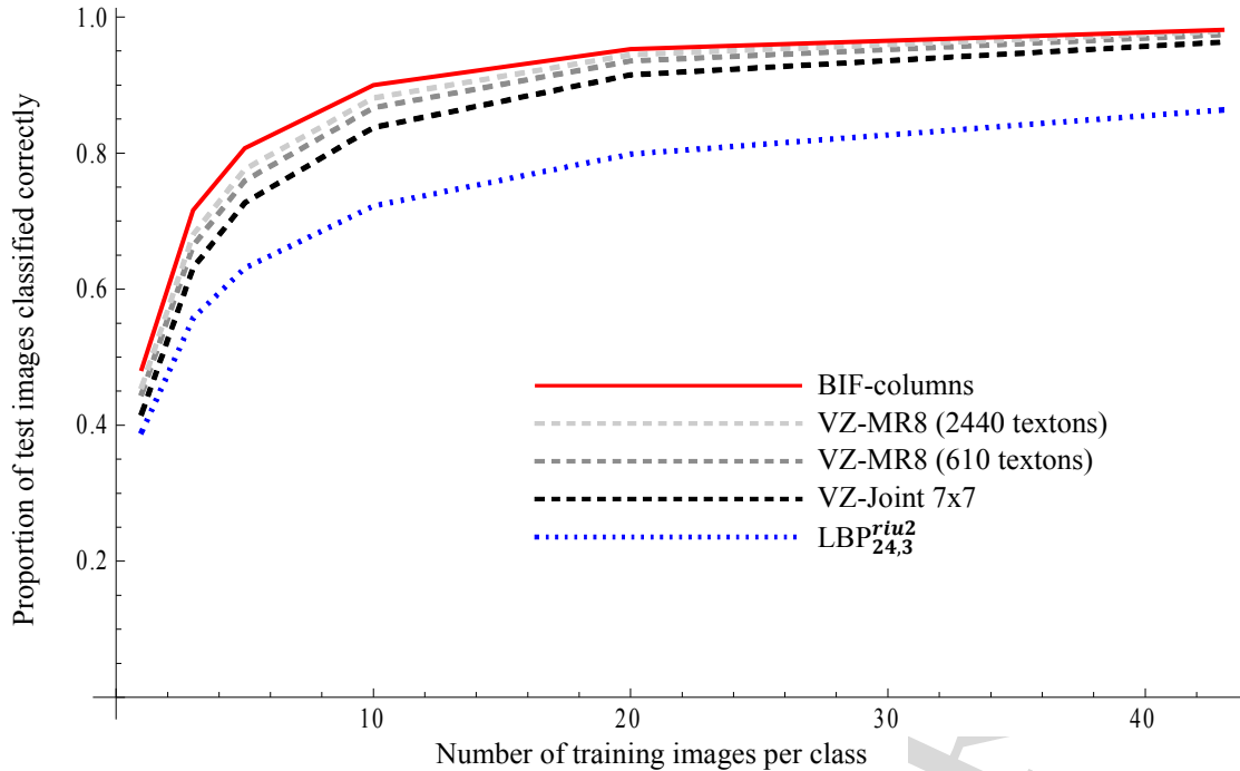
Fig. 4 The mean proportion of correctly classified images over 100 random splits of the CURET dataset into training/test data, for a range of training set sizes. The best result for BIF-columns (with 43 training images per class) is 98.1 \pm 0.3\% .
