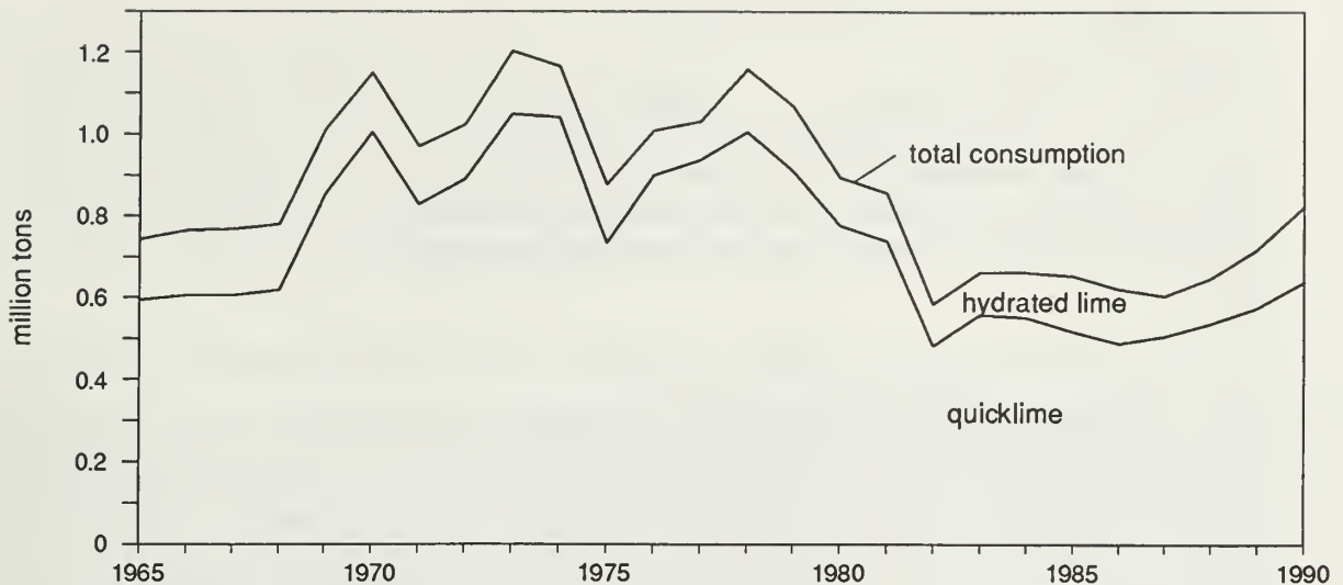
Figure 14 Trends in consumption of quicklime and hydrated lime in Illinois, 1965–90.
