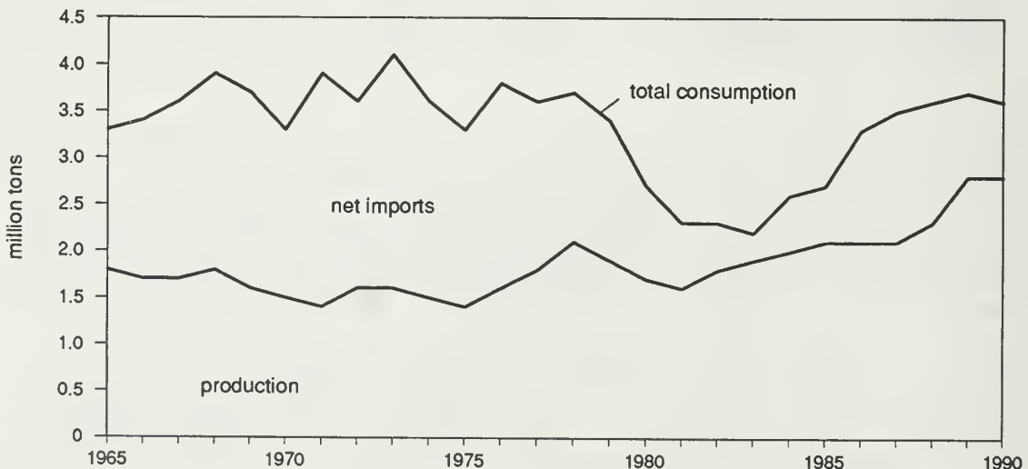
Figure 13 Production and consumption of finished Portland cement in Illinois, 1965-90.
