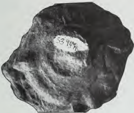
Figure 34 (upper) Conostichus stouti with 12-fold symmetry. Cone shape and basal discs have longitudinal furrows. Figure 35 (lower left) Photo shows morphology and activities of both Conostichus and Asterosoma . Figure 36 (lower right) Conostichus and Asterosoma component.
