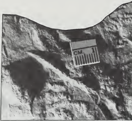
Figures 14 and 15 Trackways made by kroupichnium.
