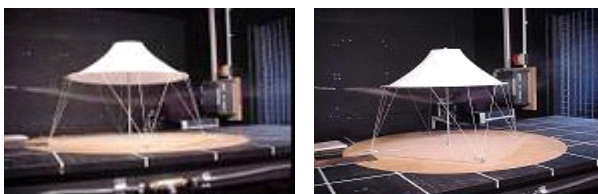
Figure 8: Visualization of airflow around conic membrane structure (wind tunnel experiment)
