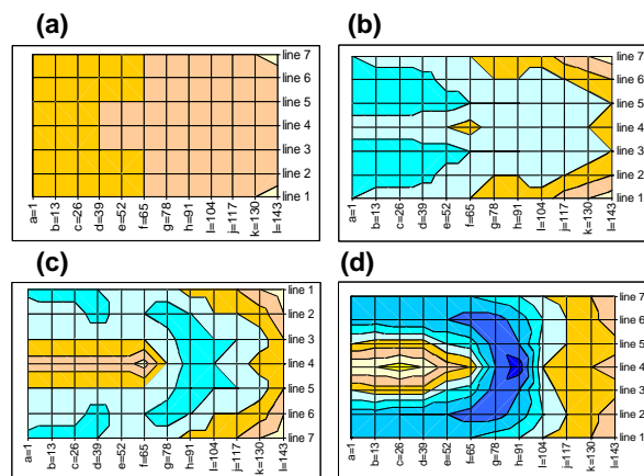
Figure 10: Airflow patterns at a height of 6.5 cm above the base for (a) no cone; (b) the circular flat disc; (c) straight closed cone at 3cm; (d) straight closed cone at 17cm high;
