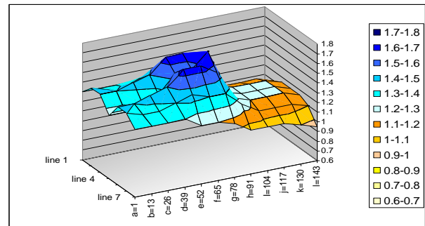
Figure 9: Air velocities (m/s) around the IC17 cone at a height of 6.5 cm above the base shown as a 3D surface (wind from the left).
