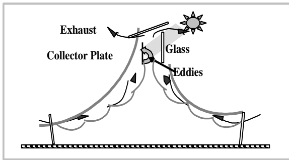
Figure 7: A solar chimney incorporated to a fabric membrane structure
