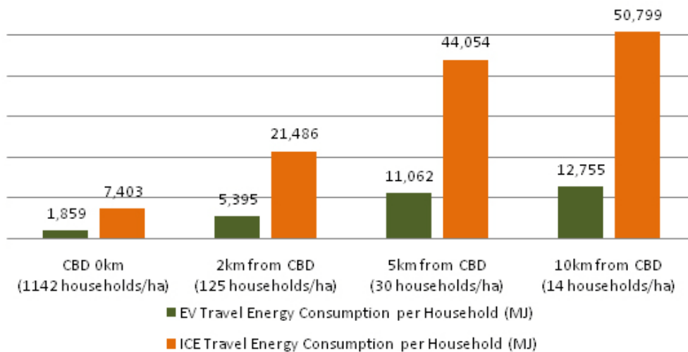
Fig. 10: Travel energy consumption comparison (MJ/household/year)
