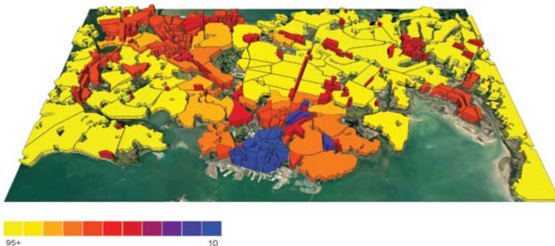
Fig. 7: Solar energy generation potential ( \text{kWh/m}^2 floor area/year).
