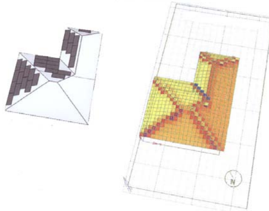
Fig. 4: Analysing the capacity of residential roofs for PVs taking account of orientation, tilt and PV module.
