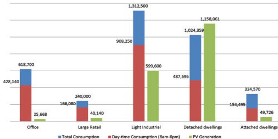
Fig. 6: Annual energy consumption of building types (day-time & total) compared with PV energy generation (kWh).
