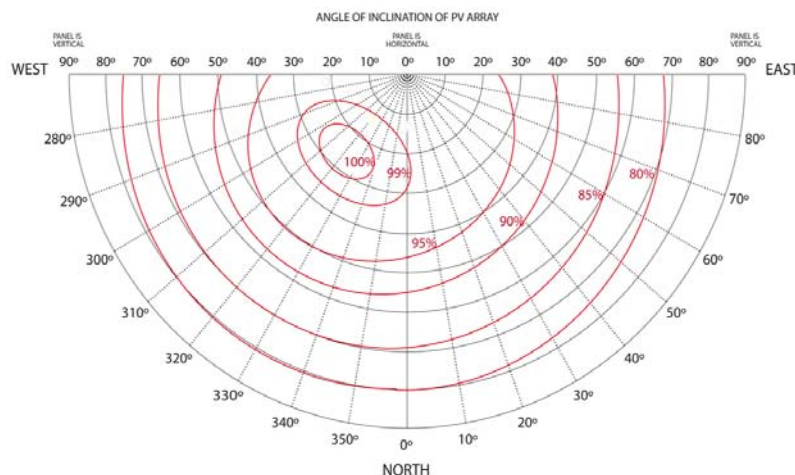
Fig. 2: Protractor for PV efficiency in Auckland, depending on orientation and tilt.
