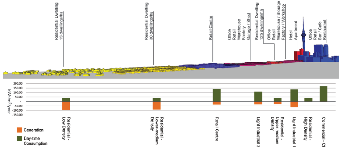
Fig. 5: Cross-section of sample showing the relative energy generation by PVs and consumption of buildings during the daytime (net-metering).
