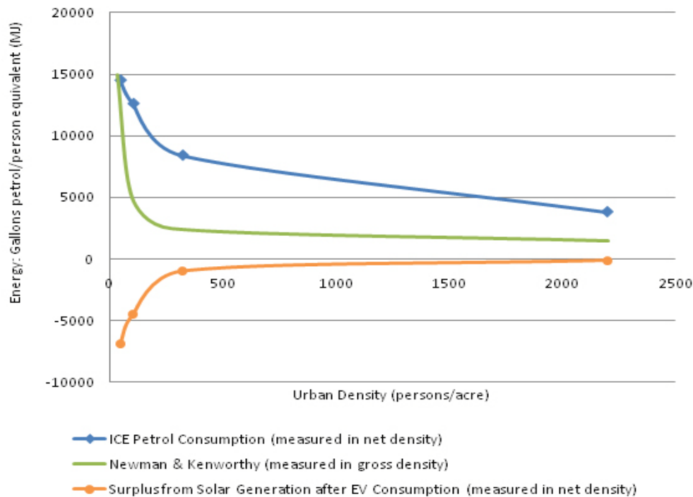
Fig. 12: The relationship between travel energy and residential density in Auckland. PVs provide enough energy to supply all household travel energy in suburbia and provide a surplus (negative figures).
