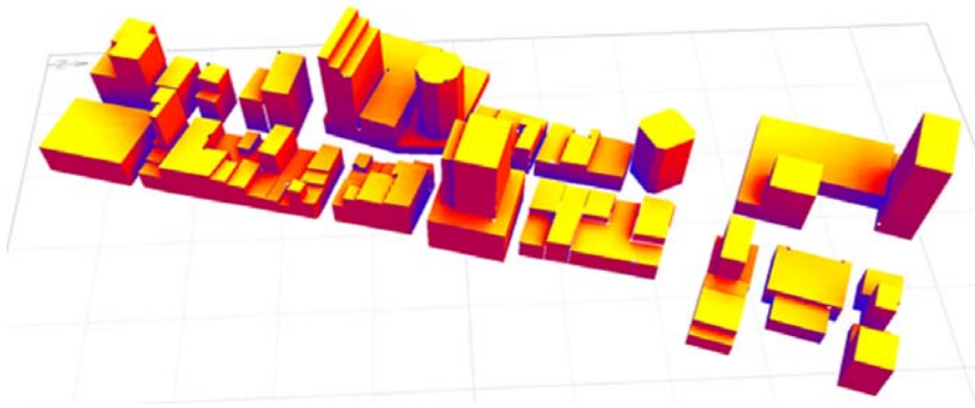
Fig. 3: Average annual solar radiation on sample of buildings in Auckland's CBD. Roofs have typically twice the radiation as walls that are unshaded or obstructed.
