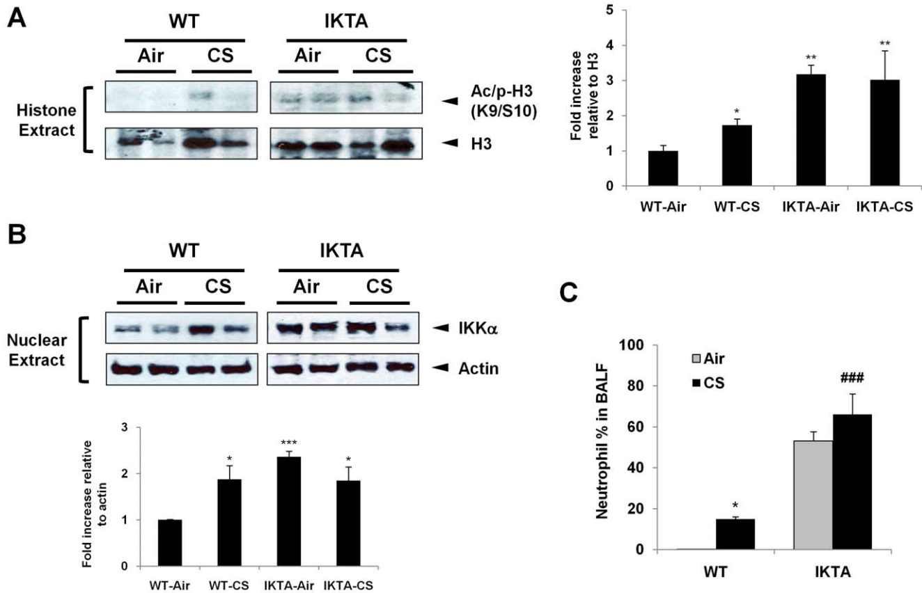
Figure 8. CS-induced histone phospho-acetylation is independent of the canonical NF-κB pathway. (A) Acid-extracted histone proteins from the lungs of IKTA mice were used for immunoblotting against phospho-acetylation of histone H3 (S10/K9). (B) Nuclear extracts were immunoblotted for IKKα levels from WT and IKTA mice exposed to air or CS. The levels of IKKα and phospho-acetylated histone H3 (S10/K9) were not augmented in lungs of IKTA mice as compared to WT mice exposed to CS. Gel pictures shown are representative of at least three separate experiments. (C) Neutrophil influx in BAL fluid of mice was determined on cytospin-prepared slides stained with Diff-Quik. After densitometry analysis, the values were normalized against the loading control, histone H3 and actin, respectively. Data shown as mean ± S.E. (n=3–5 per group). *, p<0.05, **, p<0.01, ***, p<0.001, significant compared with air-exposed WT group; ###, p<0.001, significant compared with CS-exposed WT mice. doi:10.1371/journal.pone.0023488.g008
