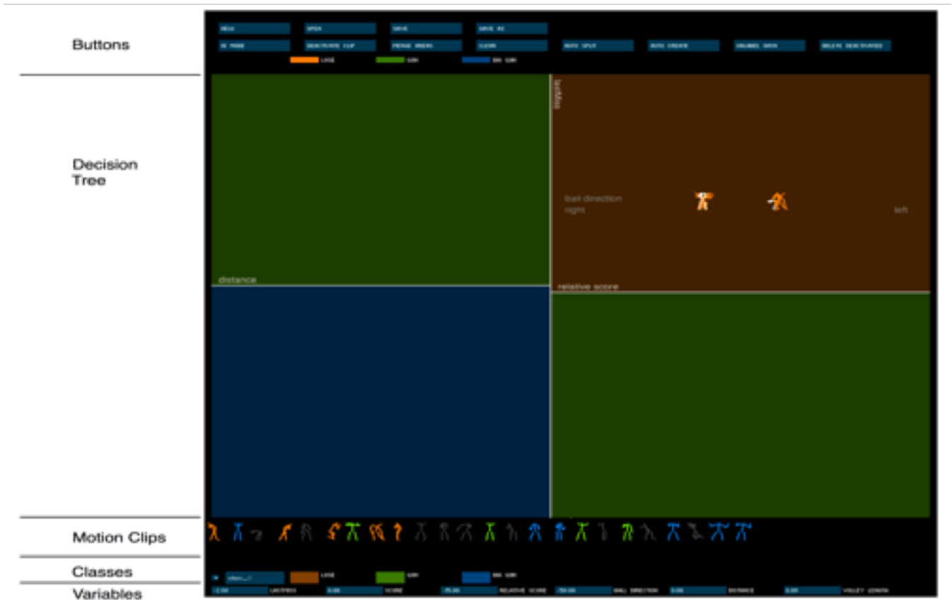
Figure 3. The interface used to design the character’s responses. As shown from bottom to top of the Figure: variables are the variables representing each point in the game. Classes are the categories defined by the player. Motion clips correspond to the body movement recorded at each point in the game. Decision tree is the interactive visualization that players use to manually edit the decision tree model. The colors in the decision tree correspond to the classes and the lines correspond to the variables.
