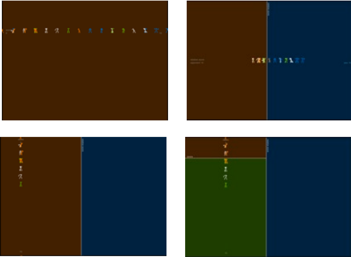
Figure 4. The decision tree visualization. Top left: the tree is empty. Hovering the mouse in the space shows the motion clip thumbnails ordered according to variable. Top right shows an internal node in the decision tree according to the selected variable. The line (i.e., threshold) can be modified by dragging it. Bottom left shows that clicking in an area selects that area and displays just those clips that are classified as belonging to that leaf node. Bottom right: the decisions are alternately split horizontally and vertically at alternate levels of the tree; so at the next level down the motion clips are displayed vertically and shift clicking results in a vertical split
