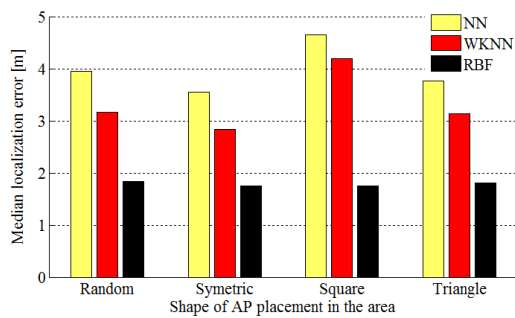
Fig. 6: Impact of the shape of APs.
