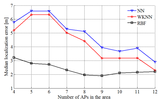
Fig. 5: Impact of the number of APs.
