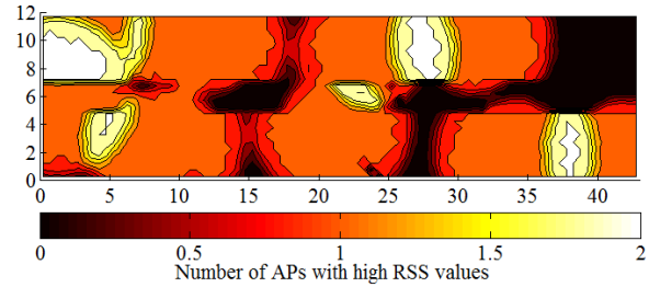
Fig. 12: Distribution of APs with RSS values higher than -65 \text{ dBm} .
