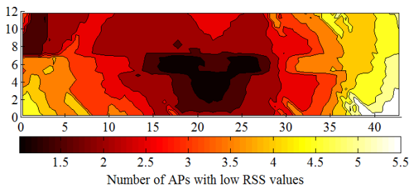
Fig. 10: Distribution of APs with RSS values lower than -85 \text{ dBm} .
