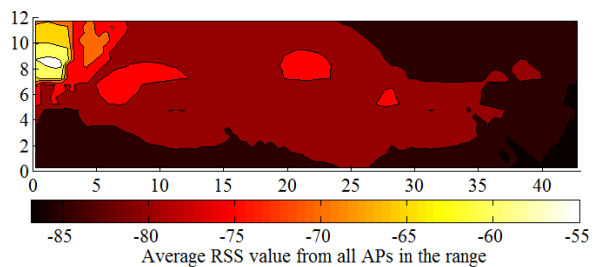
Fig. 9: Distribution of mean RSS values from all APs in the range.
