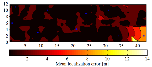
Fig. 7: Distribution of mean localization error in the area.
