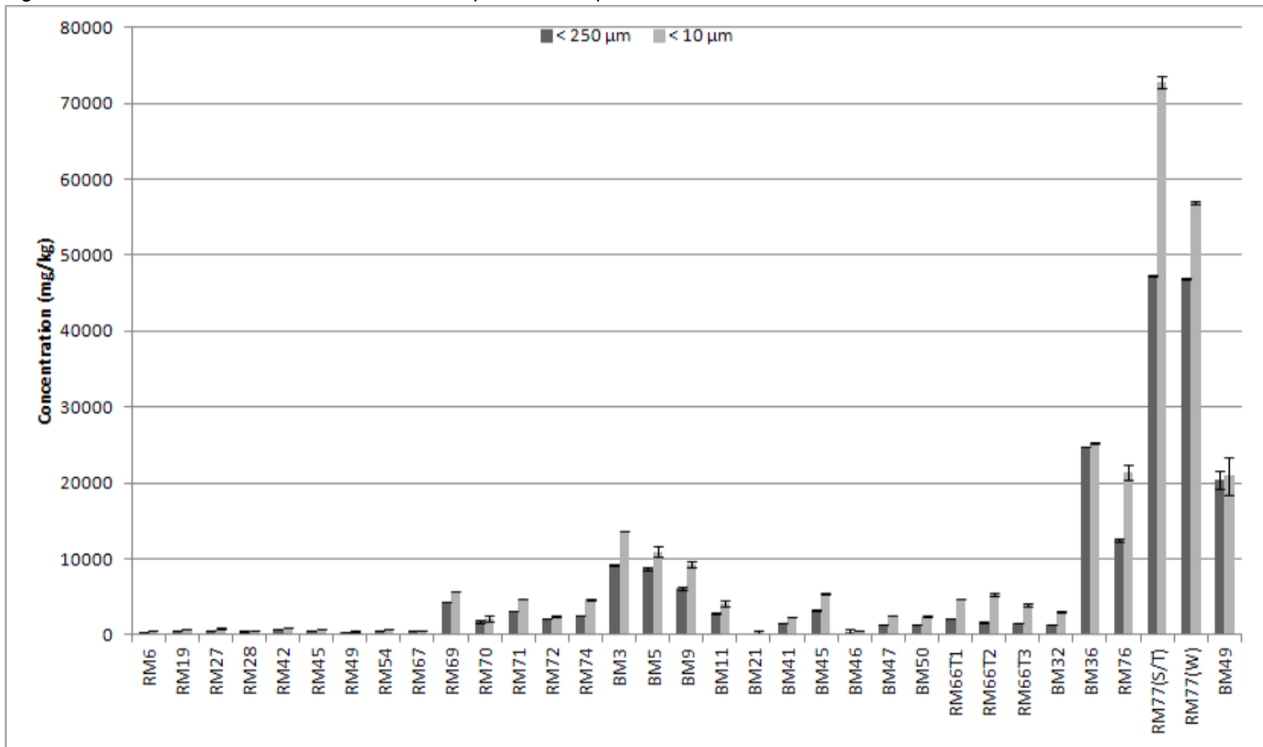
Figure 5.3: Plot of Pb total concentrations in < 250 μm and < 10 μm fractions
