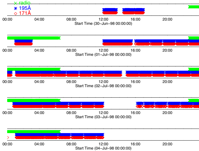
Fig. 2. Observational coverage over AR8253 by TRACE 171 Å (red) and 195 Å (blue), and NoRH 17 GHz (green) in the analysed time interval. Small gaps in EUV observations of order 100 s are due to channel switching, and large ones are due to routine observations on the solar limb (including polar regions), re-pointing or to avoid radiation belts.
