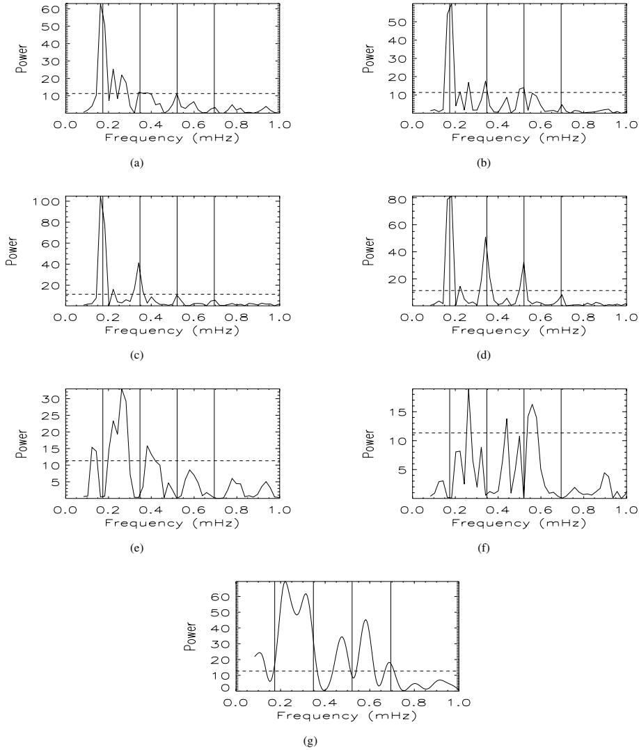
Fig. 4. a), b) Power spectra of the time series (1998-07-03 00:47–09:00 UT) of a macro-pixel ( 3 \times 3 pixels) situated along the mid-way of the slit (Fig. 1b in EUV 171 Å (left) and 195 Å (right)). c), d) The corresponding spectra of an enlarged macro-pixel ( 20 \times 20 pixels). e), f) The power spectra after filtering out the orbital frequencies. g) The power spectrum of NoRH 17 GHz radio emission, (1998-07-03 02:55–06:30 UT). The vertical dot-dot-dashed lines are the orbital frequency and its higher harmonics. A horizontal dashed line indicates the 99% confidence level in all the panels (see Sect. 2.4). The detected peaks in all the bandpasses are summarised in Table 1.
