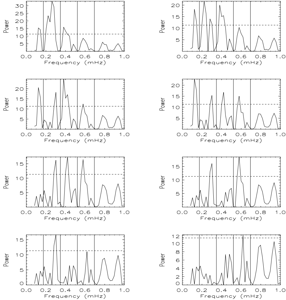
Fig. 5. Lomb-Scargle periodograms of 171 Å data shown after iteratively subtracting the highest peak in the spectrum with power above 1% of FAP (dashed line). The iteration is displayed in order from left to right, top to bottom.
