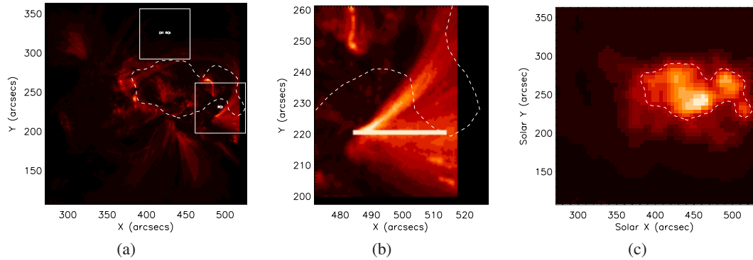
Fig. 1. a) The field of view over AR8253 taken at 1998-07-01 01:01 UT in TRACE 171 Å bandpass, the region of interest (ROI) in the white box includes the fan-like structure and is re-sized to the left, an off-ROI region including the weakest intensity area is marked to the top. b) The region of interest (128 × 128 pixels) showing the fan-like structure; a slit of the macro-pixels (3 × 3) is selected along the fan. c) The intensity map of 17 GHz radio emission over AR8253 at 1998-07-01 01:01 UT. The contour in dashed line marked the sunspot area.
