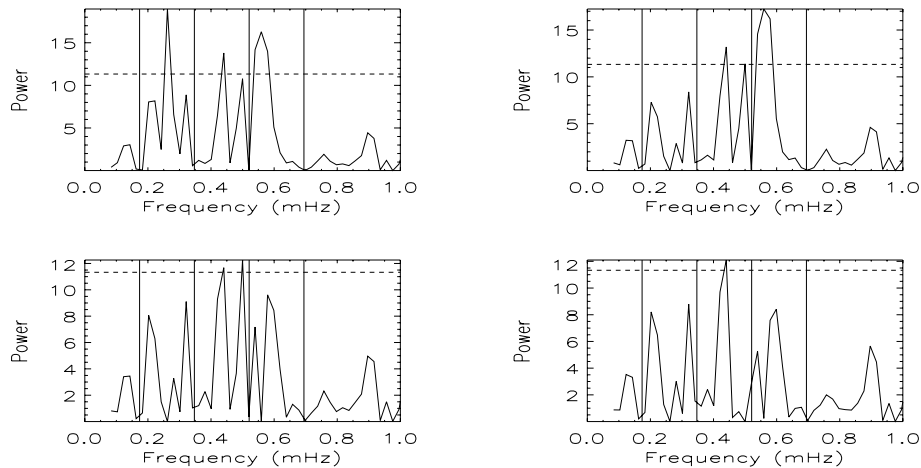
Fig. 6. The same analysis to 195 Å data as in Fig. 5. The iteration stops earlier than those for 171 Å data, but we note peaks with power below 99% confidence level, near 0.202 and 0.320 mHz, that may be of relevance.
