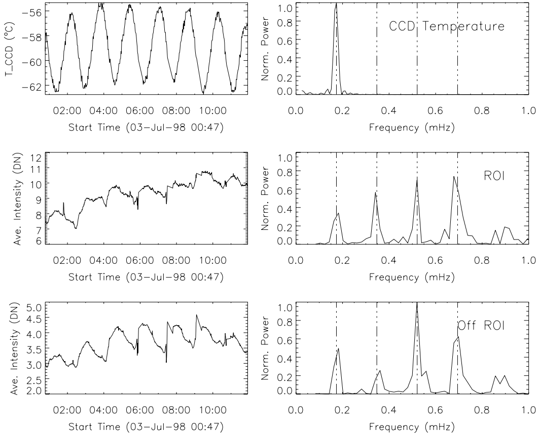
Fig. 3. Left column: time series (1998-07-03 00:47–12:00 UT). Right column: the corresponding normalised power spectra, a 30-min running average is removed from the intensity time series beforehand, the harmonics of the orbital periods are marked with the vertical dash-dot-dot lines, corresponding to the periods 96, 48, 32, 24 min. From top to bottom row: TRACE CCD temperature variation (°C), the average intensity (DN) of the ROI, and off ROI.
