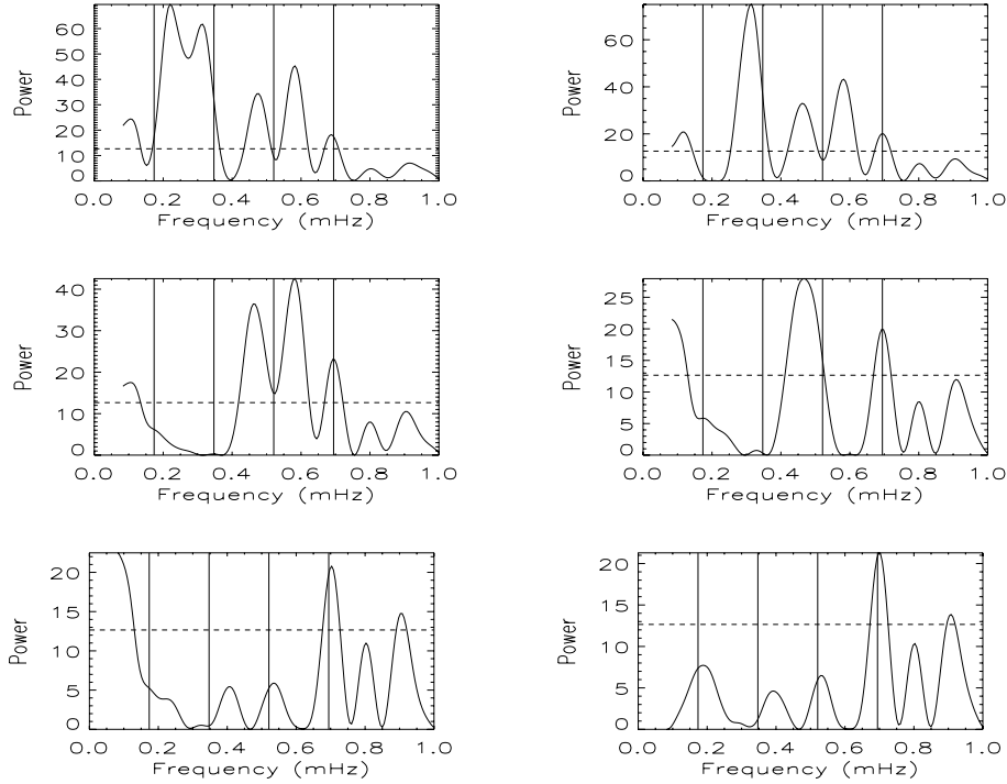
Fig. 7. The same analysis to NoRH 17 GHz data as in Fig. 5 .
