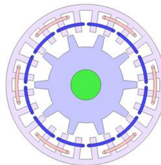
Fig. 5. 3-phase 24S-10P FEFSM
