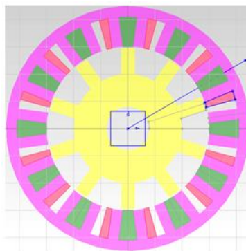
Fig. 6. Initial design of the 24S-10P FEFSM
