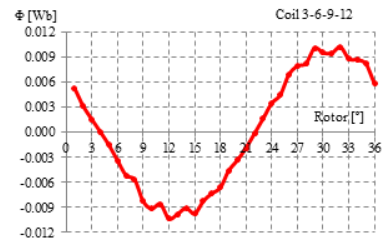
Fig. 11. Flux linkage of coil 3, 6, 9 and 12
