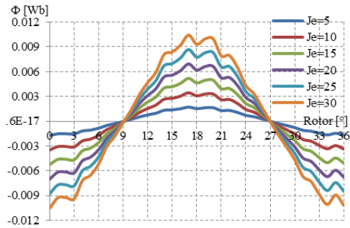
Fig. 14. U phase flux linkage at various FEC current
