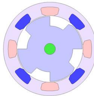
Fig. 3. 1-phase 8S-4P FEFSM.
