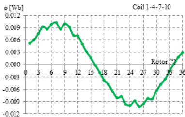
Fig. 9. Flux linkage of coil 1, 4, 7 and 10
