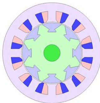
Fig. 4. 3-phase 12S-8P segmental rotor
