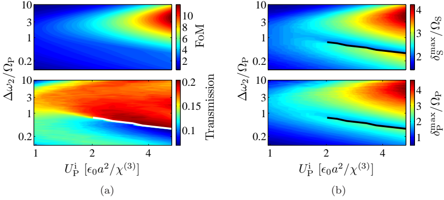
Figure 7.8: (a) Upper panel: The maximum FoM found by varying (\delta_S, \delta_P) as a function of U_P^i and \Delta\omega_2 . (a) Lower panel: The transmission of the signal, U_{So}^{1\{0\}}/U_{Si}^{1\{0\}} , corresponding to the maximum of the FoM in the upper panel. As in Fig. 7.6(a), the white line indicates a discontinuity boundary, where the transmission suddenly changes value. (b) Upper panel: The value of \delta_S^{\max}/\Omega_S corresponding to the maximum of the FoM. The discontinuity boundary is also shown with a black line. (b) Lower panel: The value of \delta_P^{\max}/\Omega_P , which corresponds to the maximum of the FoM along with the discontinuity boundary.
