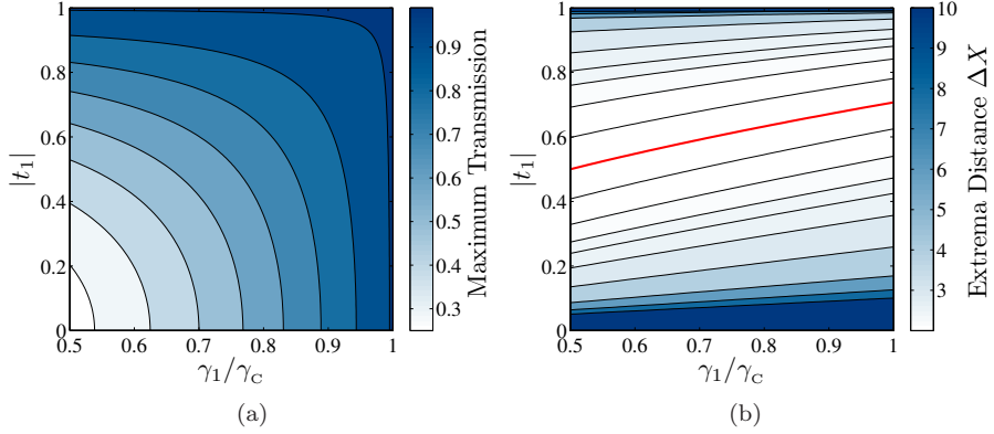
Figure 8.11: Properties of the CW transmission in Eq. (8.3.1). (a) The maximum transmission as a function of coupling rate ratio and the blockade transmittance. (b) The frequency distance between the maximum and minimum transmission. The red line shows the minimum given by |t_1| = \sqrt{\gamma_1/2\gamma_c} .
