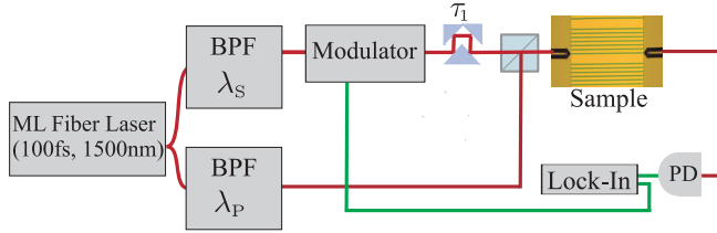
Figure 5.1: Schematic illustration of the setup for homodyne pump probe experiments with the pump and signal co-propagation through the sample. The red lines indicate the paths of optical signals, and the green show electrical signals. The variable delay line introduces a delay \tau_1 in arrival time at the cavity between the pump and the signal. ML: Mode locked. BPF: Band pass filter. PD: Photo detector.
