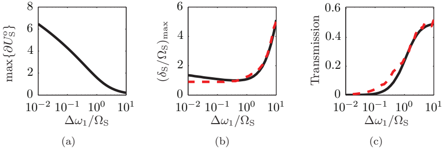
Figure 7.7: (a) The maximum value of \partial U_{\text{S}}^{\circ}(\delta_{\text{S}}/\Omega_{\text{S}}) , defined in Eq. (7.5.4), plotted as a function of the ratio between the cavity linewidth and the pulse bandwidth. (b) The value of \delta_{\text{S}}/\Omega_{\text{S}} corresponding to the maximum in (a) (solid black) and a cross section of \delta_{\text{S}}^{\text{max}}/\Omega_{\text{S}} at U_{\text{P}}^{\text{i}} = 0.105 \times \epsilon_0 a^2 / \chi^{(3)} from Fig. 7.6(a) (dashed red). (c) Transmission at the maximum in (a) (solid black) and a cross section of the transmission at U_{\text{P}}^{\text{i}} = 0.105 \times \epsilon_0 a^2 / \chi^{(3)} from Fig. 7.6(a) (dashed red).
