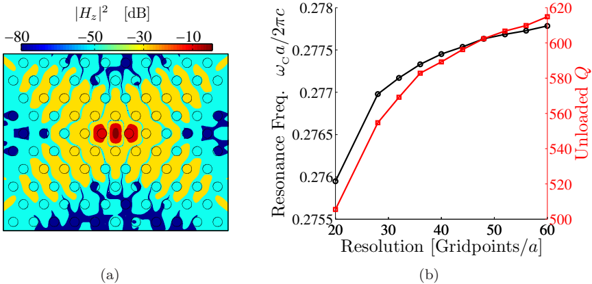
Figure B.4: Convergence test. (a) The structure considered consisting of an H0 cavity in a finite sized PC membrane. The parameters are: d = 0.8a , r = 0.23a , and \delta x = 0.16a . (b) Resonance frequency and quality factor as a function of resolution measured in grid points per lattice constant.
