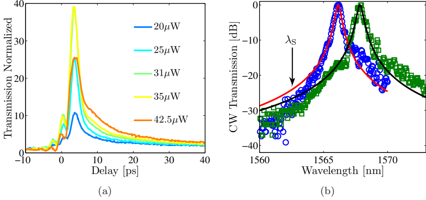
Figure 5.6: (a) Normalized signal transmission as a function of delay \tau_1 for the same sample as in Fig. 5.3 using the setup in Fig. 5.5. The signal average power is \bar{P}_s^i = 3.3\mu\text{W} and it is centered at \lambda_P = 1562.5\text{nm} . The wavelength of the pump is \lambda_P = 1565.1\text{nm} and the different curves correspond to different pump powers \bar{P}_P^i . The filter is centered at \lambda_F = \lambda_S and has a FWHM bandwidth of \Delta\lambda_F = 0.8\text{nm} . (b) CW transmission measured three months apart. The solid lines show Lorentzian fits to the measured data. A normalization is used so the peak transmission equals 1.
