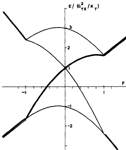
Fig. 1. The energy levels in the E + T_2 case are shown in units of G_{TX}^2/K_T as a function of F = \Delta/(4G_{TX}^2/K_T) . In all cases the levels are calculated for the configuration which minimises the energy in the ground state.
