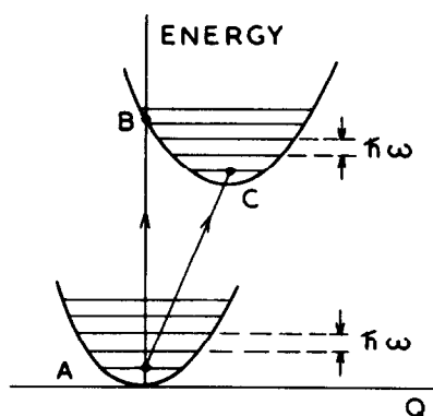
Fig. 2. Configuration coordinate diagram of a simple system with non-degenerate levels interacting with one mode Q .
