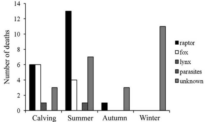
FIG. 4.—Causes of mortalities of marked saiga calves captured during 2008–2010 in western Mongolia. Spring is excluded from the graph because no mortality occurred during this period. Winter deaths are all attributed to unknown causes because monitoring did not occur during that season.
