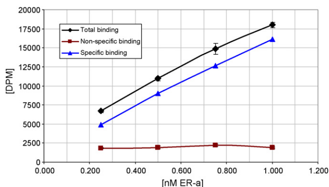
Fig. 1. Determination of the necessary receptor concentration–linear relationship between specific binding and receptor concentration. Under conditions corresponding to competitive binding increasing ER \alpha concentrations were incubated with 1 nM [ ^3 H]-17 \beta -estradiol. Non-specific binding was assessed in parallel in the presence of 1 \mu M unlabeled 17 \beta -estradiol. Following incubation overnight, unbound radiolabeled ligand was removed by absorption to dextran-bound charcoal (DBC) and sedimentation of DBC by centrifugation. ER \alpha -bound radiolabel in the supernatant was determined by liquid scintillation counting. Specific binding was calculated as the difference of total and non-specific binding. For each condition six replicates were performed. Means \pm S.D. are given.
