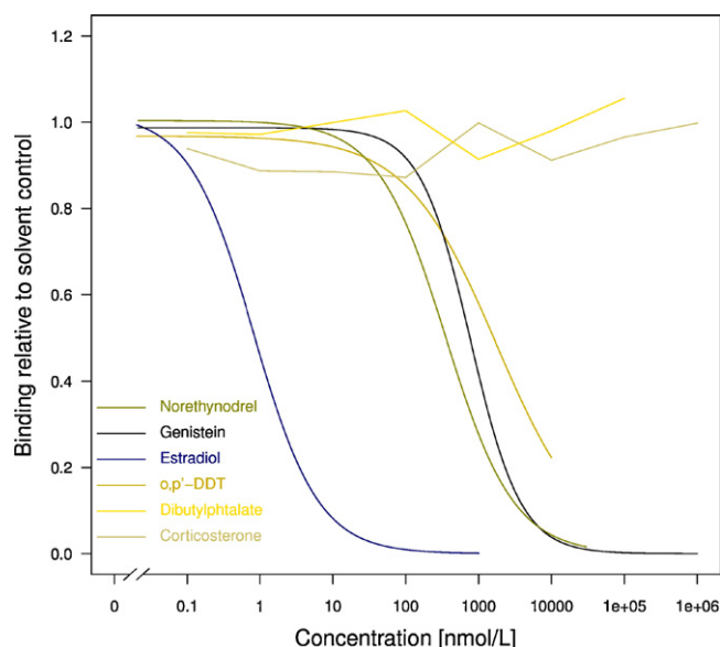
Fig. 4. Competitive binding to the human recombinant full length estrogen receptor- \alpha of reference and test compounds using DMSO as solvent. Receptor (nominally 0.5 nM) was incubated with 1 nM [ ^3 H]-17 \beta -estradiol and increasing concentrations of compounds as indicated. Following incubation overnight, unbound radiolabeled ligand was removed by absorption to dextran-bound charcoal (DBC) and sedimentation of DBC by centrifugation. Receptor-bound radiolabeled ligand in the supernatant was determined by liquid scintillation counting. Binding was corrected for non-specific binding (NSB) and expressed relative to the corresponding solvent control. Data correspond to run D. For the solvent control and for NSB in the presence of 1 \mu M 17 \beta -estradiol six replicates were performed, any other condition was studied in triplicate. Data correspond to run F. For the sake of clarity, only the curve fit, but no individual data points are given.
