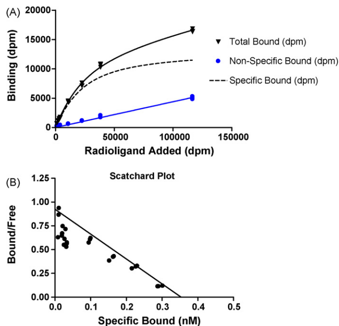
Fig. 2. (A) Saturation binding data of the human recombinant full length estrogen receptor- \alpha utilizing [ ^3 H]-17 \beta -estradiol. ER \alpha (nominally 0.5 nM) was incubated with increasing final concentrations (0.03, 0.06, 0.08, 0.10, 0.30, 0.60, 1.0, 3.0 nM) of [ ^3 H]-17 \beta -estradiol (1 nM = 39,072 dpm). Non-specific binding was determined in parallel in the presence of a 1000-fold molar excess of unlabeled 17 \beta -estradiol. For each condition three replicates were performed. Following incubation overnight, unbound radiolabeled ligand was removed by absorption to dextran-bound charcoal (DBC) and sedimentation of DBC by centrifugation. Receptor-bound radiolabeled ligand in the supernatant was determined by liquid scintillation counting. Specific binding was calculated as the difference of total and non-specific binding. Graphs were generated using the non-linear regression software program Prism version 5.02. The figure shows a representative experiment. (B) Scatchard analysis of the human recombinant full length estrogen receptor- \alpha utilizing [ ^3 H]-17 \beta -estradiol. Data for total and non-specific binding shown in (A) were analysed by Prism version 5.02 taking into account ligand depletion. The figure shows a representative experiment.
