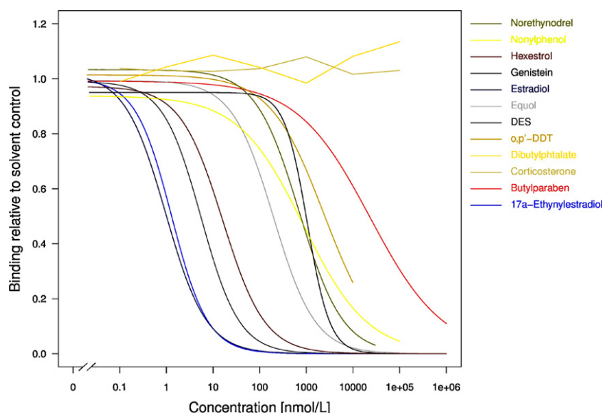
Fig. 3. Competitive binding to the human recombinant full length estrogen receptor- \alpha of reference and test compounds using ethanol as solvent. Receptor (nominally 0.5 nM) was incubated with 1 nM [ ^3 H]-17 \beta -estradiol and increasing concentrations of compounds as indicated. Following incubation overnight, unbound radiolabeled ligand was removed by absorption to dextran-bound charcoal (DBC) and sedimentation of DBC by centrifugation. Receptor-bound radiolabeled ligand in the supernatant was determined by liquid scintillation counting. Binding was corrected for non-specific binding (NSB) and expressed relative to the corresponding solvent control. For the solvent control and for NSB in the presence of 1 \mu M 17 \beta -estradiol six replicates were performed, any other condition was studied in triplicate. Data correspond to run D. For the sake of clarity, only the curve fit, but no individual data points are given.
