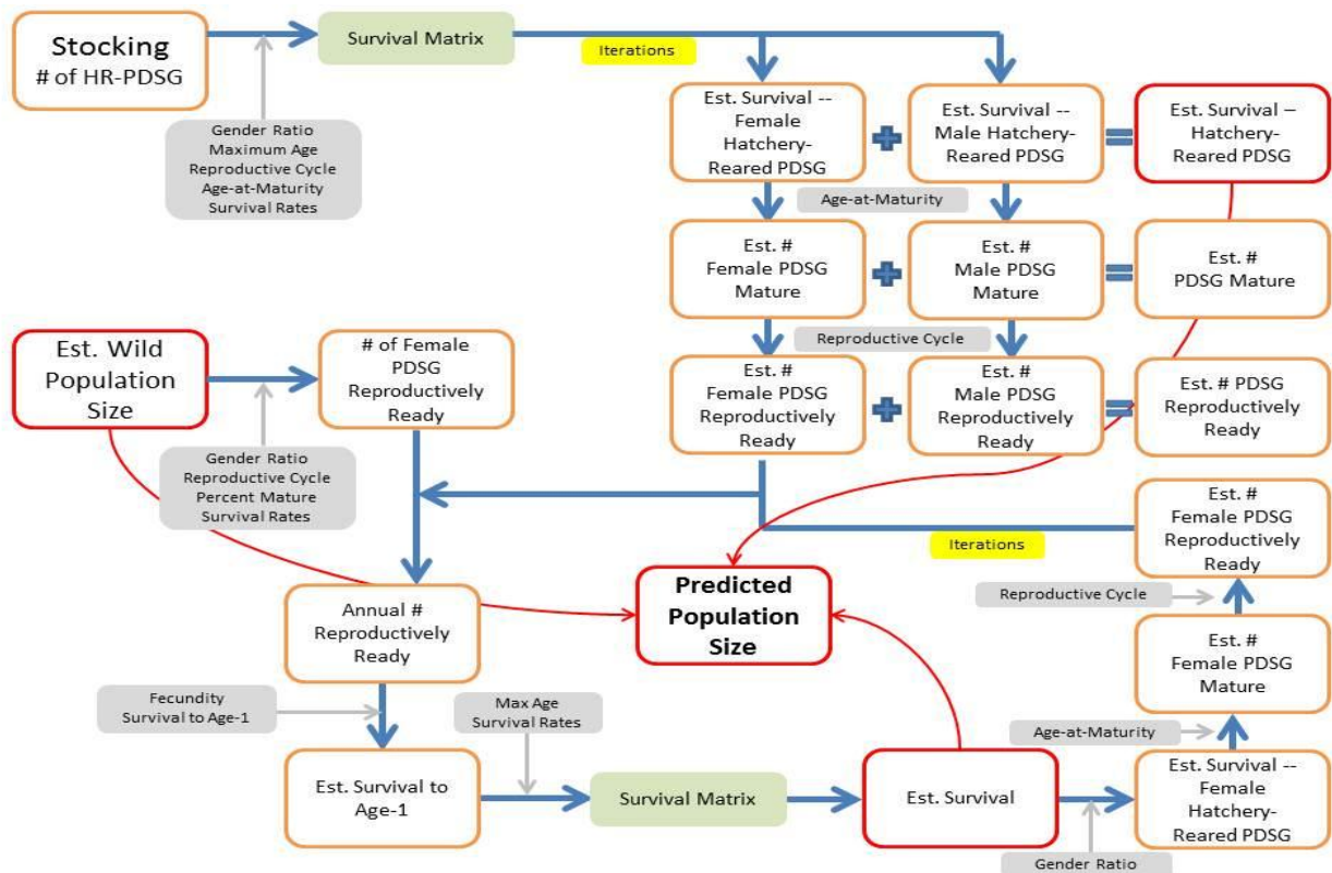
Figure 3-1. Conceptualization of the population viability analysis (PVA) model for the lower Missouri River. Open boxes are input parameters gathered from published and unpublished data while the gray boxes represent input parameters that can be adjusted within the model.
