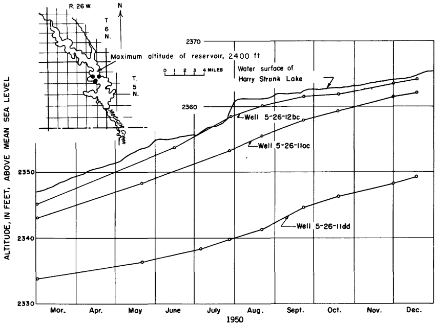
Figure 80. —Comparison of the water surface of Medicine Creek Reservoir with the water level in nearby wells.
