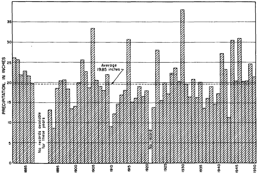
Figure 77. —Precipitation at McCook, 1882-1950. (From records of the U. S. Weather Bureau)
