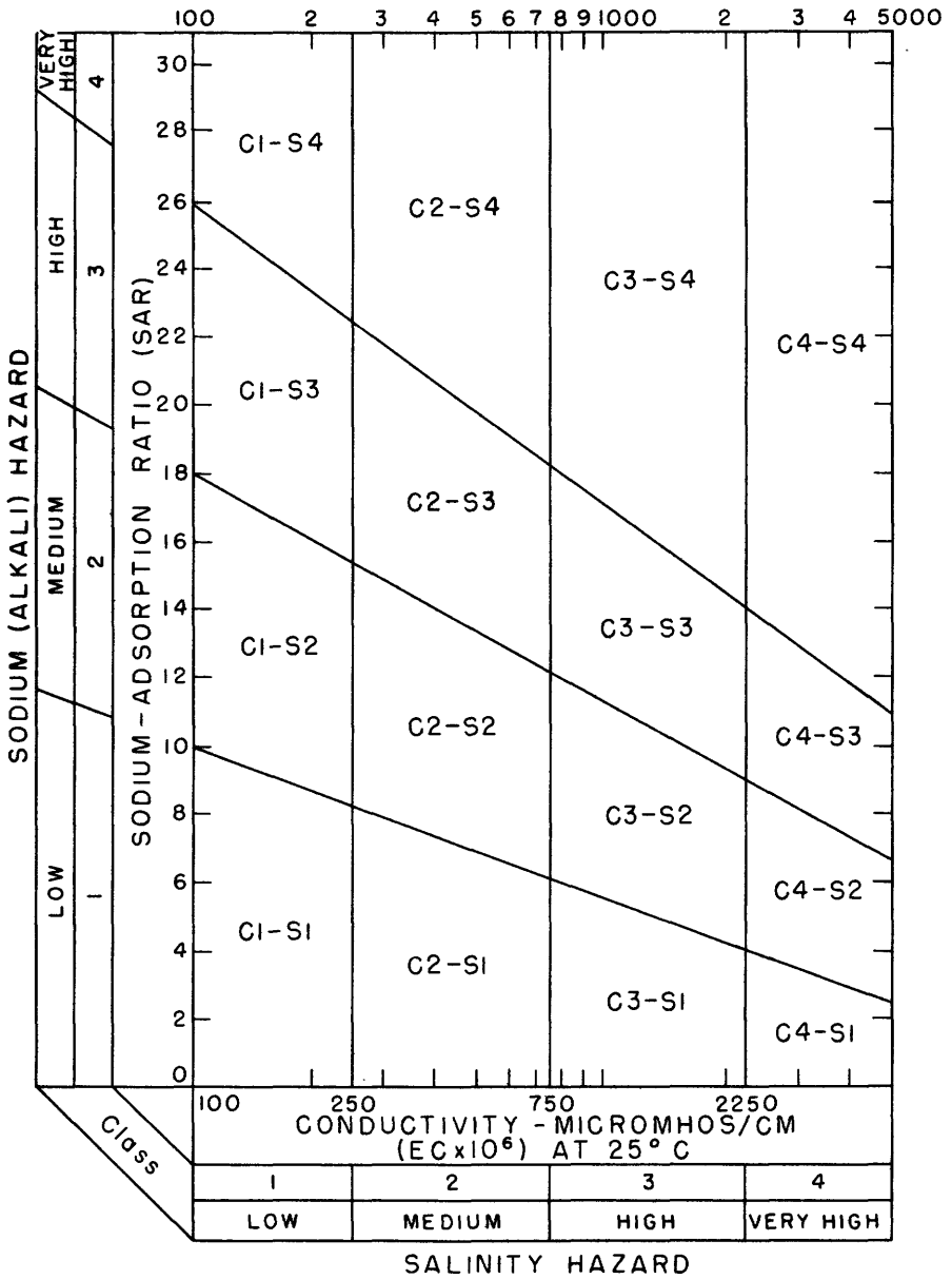
Figure 81. —Classification of irrigation water (After U. S. Salinity Laboratory Staff, 1954)
