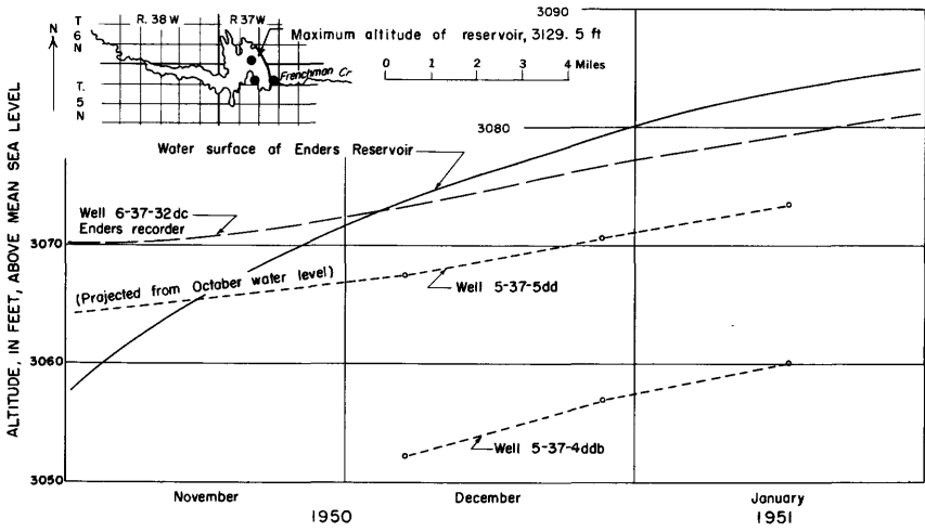
Figure 79. —Comparison of the water surface of Enders Reservoir with the water level in nearby wells.
