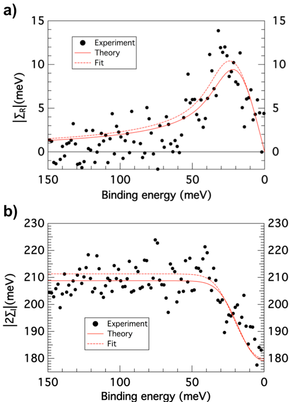
Figure 7.5: The real part (a), and the imaginary part (b) of self-energy for the surface resonance band with k_F = 0.64 \text{ \AA}^{-1} . The experimental data points ( \bullet ) for \Sigma_R are obtained from the deviation of the ARPES peak positions from the expected unrenormalized band dispersion (see Figure 7.3a) and those for \Sigma_I are obtained from the (energy) width of the photoemission peaks as described in the text. For the theoretical part, the self-energy due to electron-phonon coupling are obtained from the calculated isotropic Eliashberg function at T = 60 \text{ K} and plotted as solid curves. The calculated \Sigma_I is rigidly shifted up by
