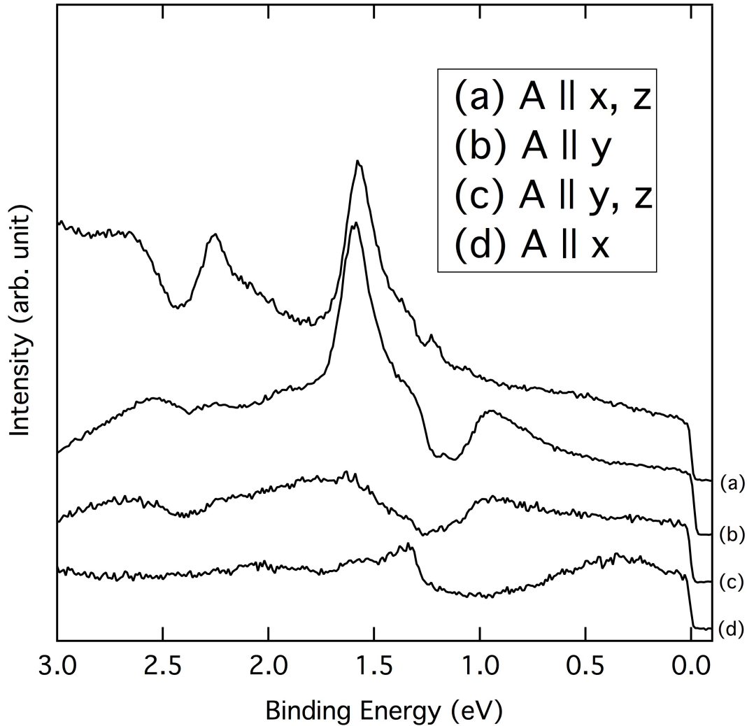
Figure 6.6: The energy distribution curves (photoemission intensity vs. binding energy) at \bar{\Gamma} for the four different incident light polarization geometry. The data are obtained by integrating the ARPES spectra in Figure 6.2 (b), (e) and Figure 6.3 (b), (e) over \pm 0.01 \text{ \AA}^{-1} . The non-vanishing component(s) of vector potential A for the four incident light polarization geometries are; (a) x - and z -component (b) y -component, (c) y - and z -component, (d) x -component.
