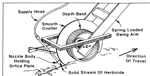
Fig. 1—Nozzle and coulter arrangement used for slot injection of herbicides.
