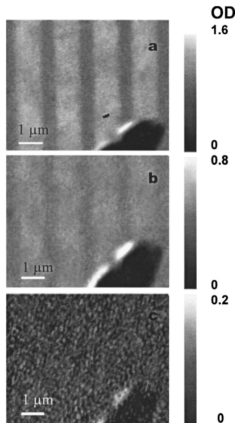
FIG. 4. Transverse xy images (absorption mode) of the patterned PTBOCST sample at (a) 290.5 eV, (b) 314.0 eV, and (c) 280.0 eV. Acquisition time of a 10\ \mu\text{m} \times 10\ \mu\text{m} image (not shown fully) was 8 min, with a dwell time of 1.6 ms per 50 nm scan distance. The dark spot in the lower right-hand corner is a hole in the sample where the incident photon flux I_0 is measured.
