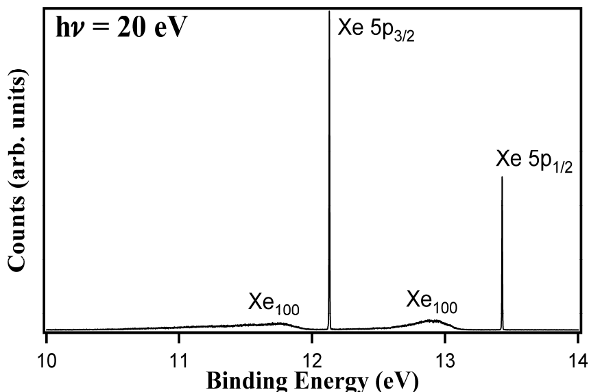
FIGURE 1. Photoelectron spectrum of Xe and clusters with average size of 100 atoms produced in supersonic jet expansion measured with a photon energy of 20 eV. The experimental resolution, as determined from the width of the 5p_{3/2} line, is 8 meV
