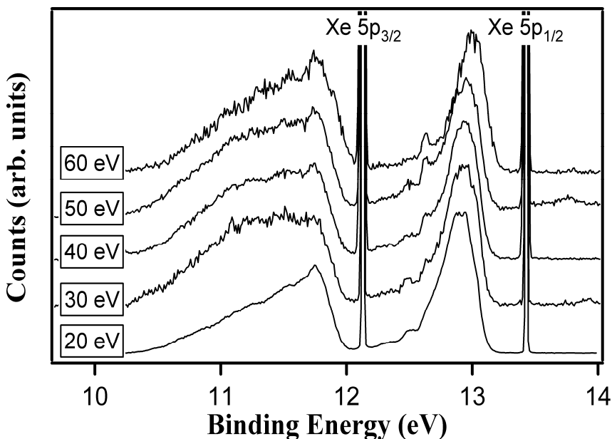
FIGURE 3. Photoelectron spectra of Xe 5p region measured at several different photon energies as indicated on the figure. The intensities were arbitrarily scaled to give the Xe 5p_{1/2} cluster lines the same intensities in all of the spectra.
