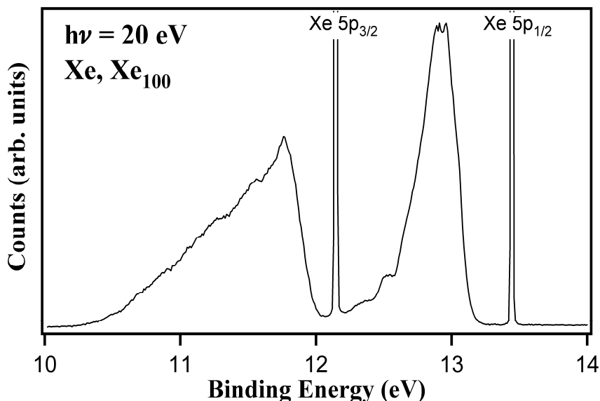
FIGURE 2. Photoelectron spectrum of Xe and clusters measured with a photon energy of 20 eV vertically zoomed to enhance the intensity of the cluster peaks. The experimental resolution, as determined from the width of the 5p_{3/2} line, is 18 meV
