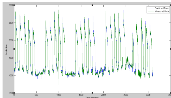
Fig. 6. Deviation of Predicted and Measured Energy data
