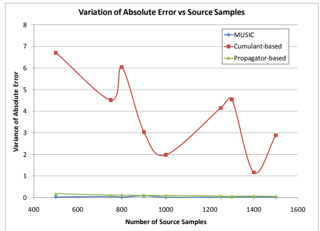
Figure 4: Effect of number of source samples on variance of estimation error of angle of arrival
