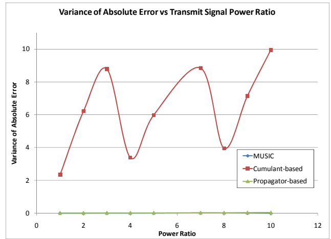
Figure 8: Effect of transmit signal power ratio on variance of estimation error of angle of arrival
