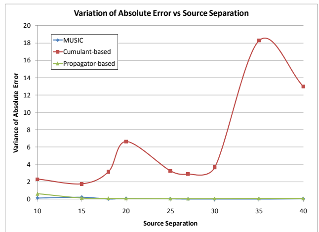
Figure 6: Effect of source separation on variance of estimation error of angle of arrival
