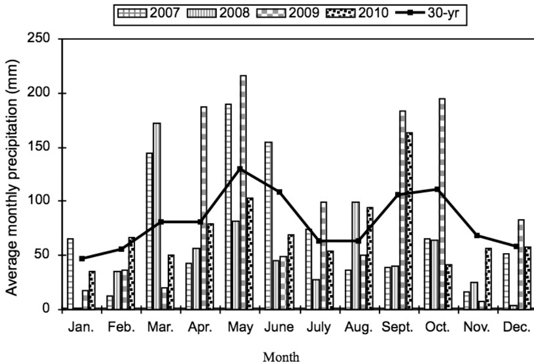
Figure 1. Monthly rainfall (mm) for the 2007 to 2010 growing seasons at Ardmore, OK, compared to the 30-yr average.
