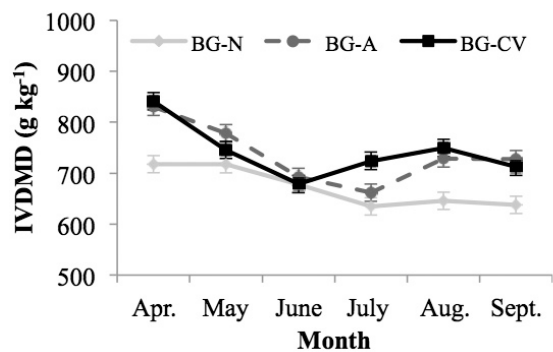
Figure 3. Seasonal changes in crude protein, acid detergent fiber (ADF), and in vitro dry matter digestibility (IVDMD) for the bermudagrass plus 112 kg N ha -1 from urea (BG-N), bermudagrass interseeded with alfalfa (BG-A), and bermudagrass interseeded with clover and vetch (BG-CV) systems averaged across the 2008, 2009, and 2010 growing seasons.
