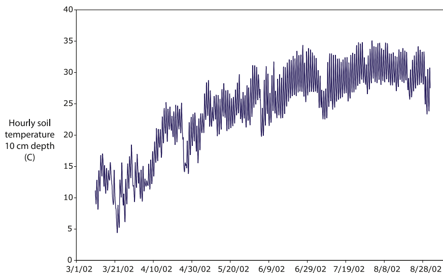
Fig. 5. Hourly soil temperature, measured at a depth of 10 cm, showing daily (diurnal) cycles and an overall seasonal pattern of gradual warming from late winter to summer.
