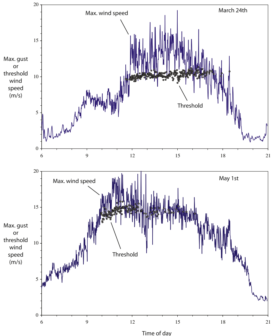
Fig. 9. Example calculations of threshold are shown for two strong wind events that occurred on 24 March and 1 May 2002. Values of threshold are represented by dots and maximum wind speed is plotted as a time series.
