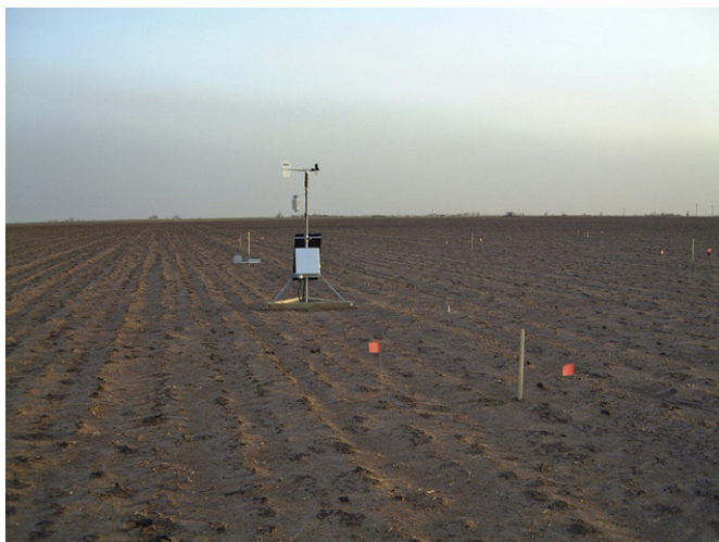
Fig. 2. Sampling system used to measure wind erosion activity and meteorological conditions on the burned field. Photo was taken the day after the fire on 12 March 2002.
