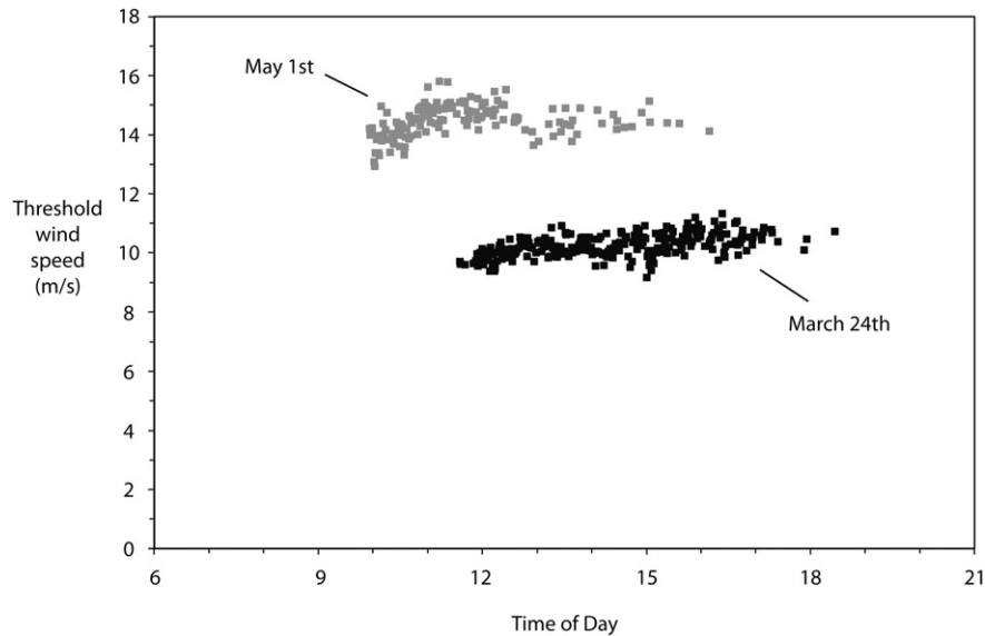
Fig. 10. Comparison of threshold values calculated for 24 March and 1 May 2002. Note the clear separation between a significantly lower threshold of 24 March and an appreciably higher threshold of 1 May 2002.
