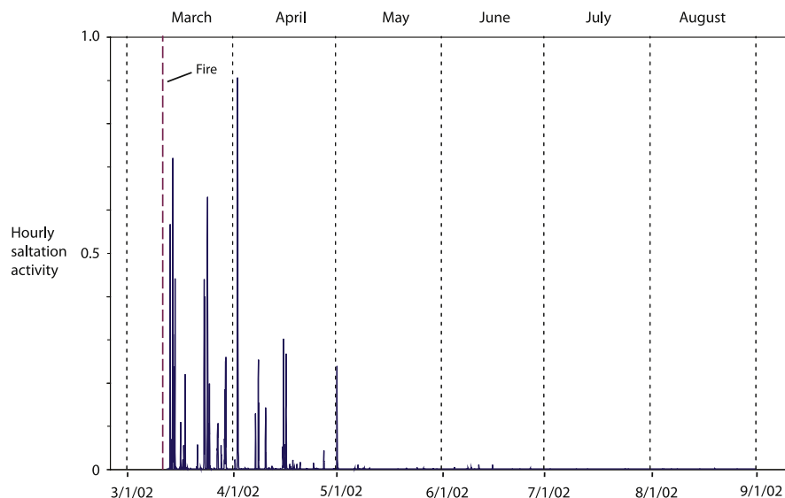
Fig. 6. Dimensionless saltation activity values plotted as a time series. A red dashed line marks the time of the fire. (For interpretation of the references to color in this figure legend, the reader is referred to the web version of this article.)
