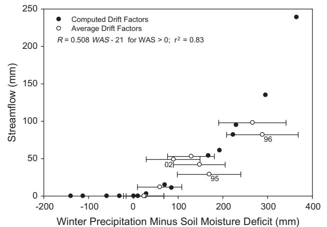
Fig. 7. Measured streamflow versus water available for sub-surface flow, defined as drift-adjusted winter–spring precipitation minus the simulated soil moisture deficit at the beginning of the water year. Points are plotted to distinguish years where drift factors were computed from those where average drift factors were used; error bars denote uncertainty associated with one standard deviation in the average drift factor. Labeled points refer to years discussed in the text.
