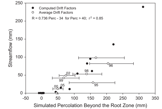
Fig. 6. Measured streamflow versus simulated percolation beyond the root zone using the SHAW model. Points are plotted to distinguish years where drift factors were computed from those where average drift factors were used; error bars denote uncertainty associated with one standard deviation in the average drift factor. Labeled points refer to years that are discussed in the text.
