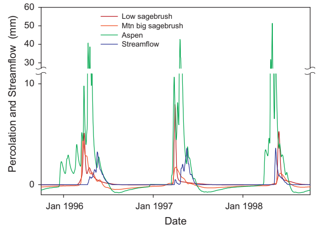
Fig. 8. Simulated percolation beyond the root zone for each landscape unit and measured streamflow for three selected water years.
