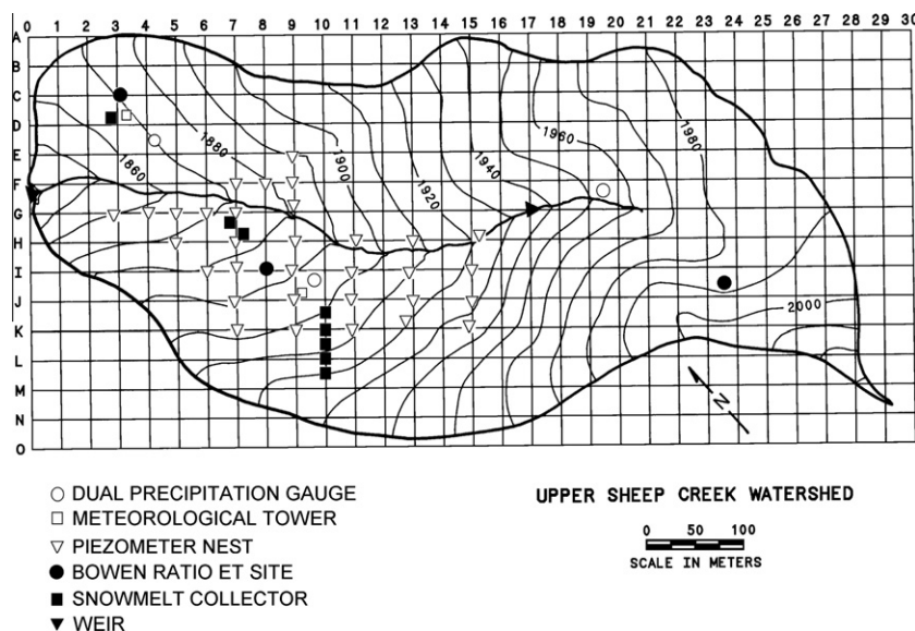
Fig. 1. Upper Sheep Creek catchment orientation, elevation range, and instrumentation.
