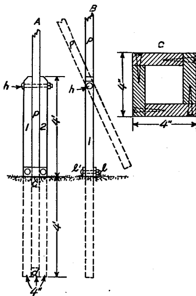
FIG. 7.—Martin-house pole. A and B : The supports (1 and 2) are 8 feet long and 4 inches square. They are held in alignment by the 4-inch blocks c and d and are buried 4 feet in the ground. A heavy bolt or section of pipe ( h ) serves as a hinge, and the base of the pole is held in position by the two hardwood blocks or iron plates ( l and l' ) bolted together. C : Cross-section of pole built of seven-eighths-inch hardwood. In case of large houses the pole and supporting posts should be 6 inches in outside diameter.
