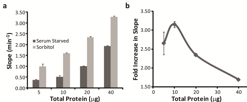
Supplementary Figure S5. The effect of the amount of lysate used in the assay on the rate of phosphorylation of MEF2A-CSox. a) Reactions conducted with 1 \mu\text{M} substrate and the indicated amount of serum starved and sorbitol-stimulated HeLa lysates. b) The fold change in reaction slope between sorbitol-stimulated and serum starved lysates with respect to the amount of lysate used in the assay. The assay is most sensitive when 10 \mu\text{g} of lysate is used. Presumably the sensitivity of the assay decreases with increasing concentrations of lysate due to the increasing amounts of off-target kinases. All reactions contained 1 \mu\text{M} staurosporine.
