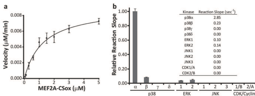
Figure 2. MEF2A-CSox is a substrate for recombinant p38 \alpha . a) Direct fit of a velocity versus MEF2A-CSox concentration plot using the Briggs-Haldane equation. b) Phosphorylation reactions were conducted with the indicated recombinant kinase (15 nM) using 1 \mu M substrate and demonstrate that MEF2A-CSox is selective for p38 \alpha among these kinases. The inset shows the average reaction slope for each kinase.
