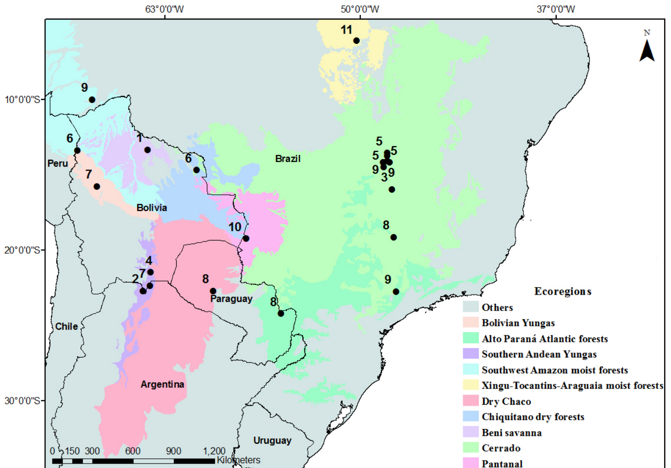
FIGURE 1. Known localities for Monodelphis kunsii and their respective ecoregions according to Olson et al. (2001). The numbers represent the chronological order of the records (i.e. 1- Pine 1975, the type locality; 2- Anderson 1982; 3- Mares et al. 1989; 4- Salazar et al. 1994; 5- Carvalho et al. 2002; 6- Vargas et al. 2003; 7- Jayat and Miotti 2005; 8- Sancha et al. 2007; 9- Pine and Handley 2008; 10- Godoi et al. 2010; 11- This work). A list of all records appears in Appendix 1.
