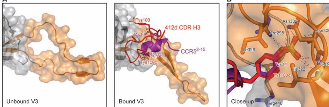
Fig. 4. A conserved site for binding sulfotyrosine on HIV-1 gp120. (A) Alterations of the V3 base to accommodate binding of sulfotyrosine. The gp120 (gray) region around the V3 loop (orange) is illustrated in ribbon diagram, with an overlying semitransparent surface for unbound (left panel) and bound (right panel) conformations. Binding of the CCR5 N terminus
