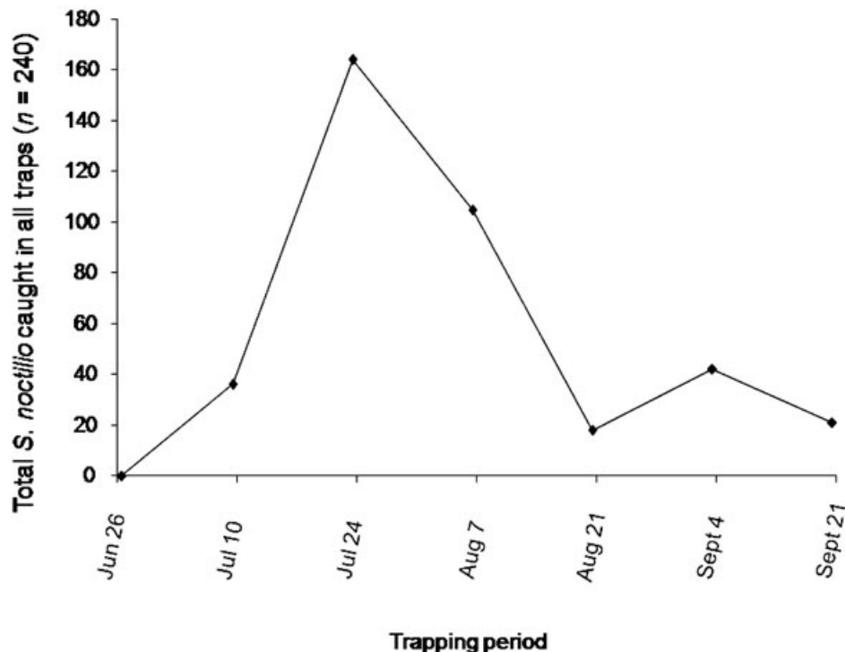
Figure 1 Total number of S. noctilio caught in all traps ( n = 240 ) in 2007. Dates represent the final day of each 2-week trapping period.
