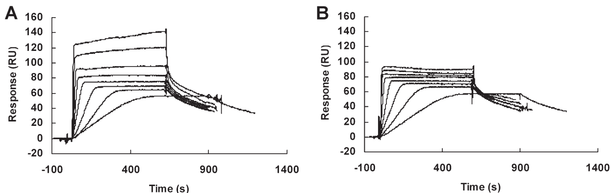
Figure S1. Comparison of surface and noncognate dsDNA-coated reference cell subtraction methods. SPR sensorgrams of different concentrations of the AtSPL14-SBP domain protein (3.125, 6.25, 12.5, 25, 50, 100, 200 and 300 nM; bottom to top) injected onto a SA sensor chip coated with a representative 156 bp cognate dsDNA fragment identified by SELEX that bound in EMSA competition assays. Binding data were collected at a flow rate of 25 \mu L/min. A) Sensorgram with signals from the control surface reference cell (no DNA) subtracted. B) Sensorgram with signals from the control reference cell (coated with a noncognate dsDNA) subtracted.
