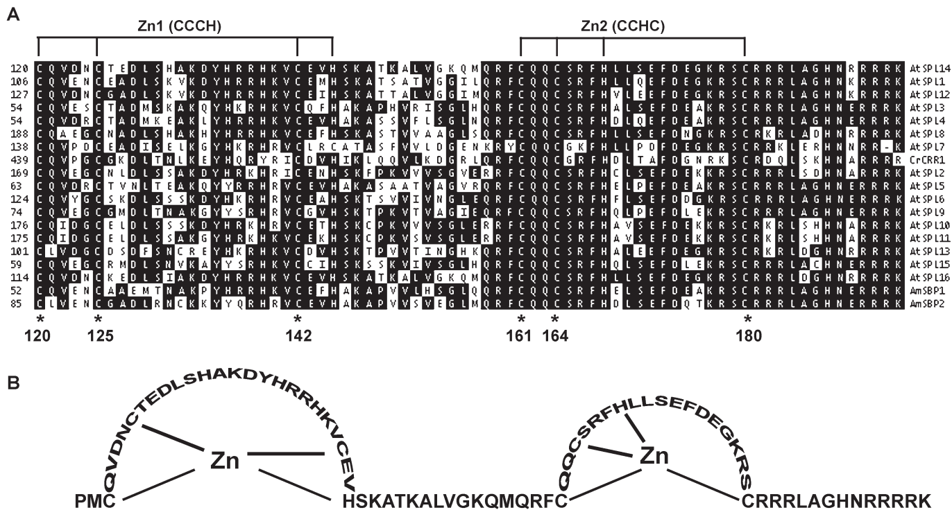
Figure S2. Multiple sequence alignment of several SBP DNA-binding domains and Zn 2+ ion coordination. A) SBP domain sequences were aligned using the Clustal method with DNASTar software (Madison, WI). Residues that match the consensus sequence are shaded in black, numbers on the left refer to the starting amino acid, protein designations are indicated on the right (organisms: At, Arabidopsis thaliana ; Cr, Chlamydomonas reinhardtii ; and Am, Antirrhinum majus ), and asterisks and amino acid numbers indicate the positions of the six highly conserved cysteines that were mutated in the AtSPL14 SBP domain. B) The coordinating Cys and His residues for Zn 2+ ions are indicated for the Zn1 (CCCH) and Zn2 (CCHC) structures.
